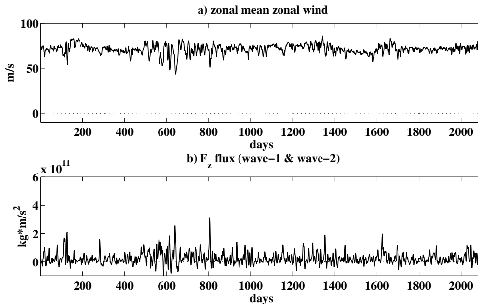
Figure 4-2: Control run: a) Representative part of the time series of zonal mean zonal wind at 60^\circ\text{S} and 10 hPa in \text{ms}^{-1} . b) Latitudinally integrated vertical component of the EP flux as described in the text for the sum of wave-1 and wave-2 at 96 hPa for the same time period, integrated between 20^\circ and 70^\circ\text{S} as given by Equation (4.1).
