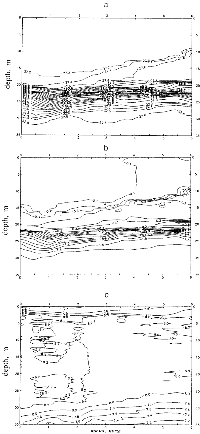
Fig. 43: Temporal variability of (a) salinity (ppt), (b) temperature (°C) and (c) dissolved oxygen (mg/l) by means of CTD-sounding at the long-term station PM 9413 (75° 30' N, 126° 00' E, September 5, 1994).
