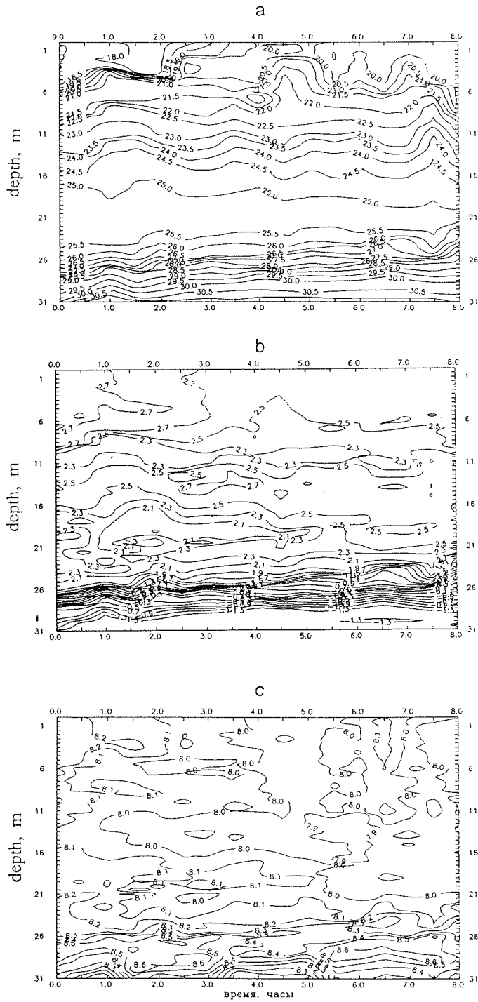
Fig. 46: Temporal variability of (a) salinity (ppt), (b) temperature (°C), dissolved oxygen (ml/l) by means of CTD-sounding at the long-term station Nb 45 (74° 30' N, 127° 30' E, September 10 - 11, 1994).
