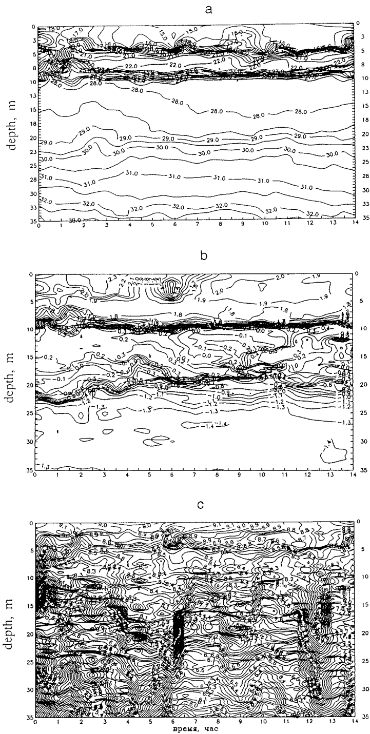
Fig. 58: Temporal variability of (a) salinity (ppt), (b) temperature ( ^{\circ}\text{C} ) and (c) dissolved oxygen (ml/l) obtained by means of CTD-soundings at the long-term station PM 94K12 ( 74^{\circ} 30' \text{ N} , 126^{\circ} 35' \text{ E} , August 23 -24, 1994).
