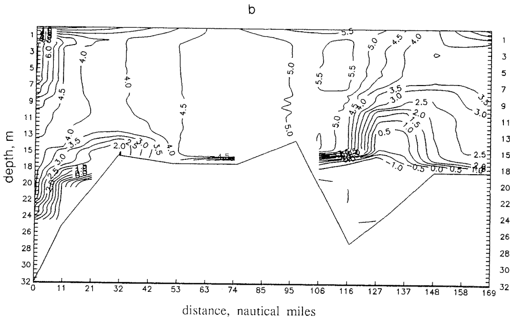
Fig. 17: Distribution of (a) salinity (ppt) and (b) temperature ( ^{\circ}\text{C} ) along the transect Dikson Island - Bely Island, Kara Sea, from 73^{\circ} 35' \text{ N} , 80^{\circ} 01' \text{ E} to 73^{\circ} 50' \text{ N} , 70^{\circ} 15' \text{ E} (September 13 - 15, 1994).
