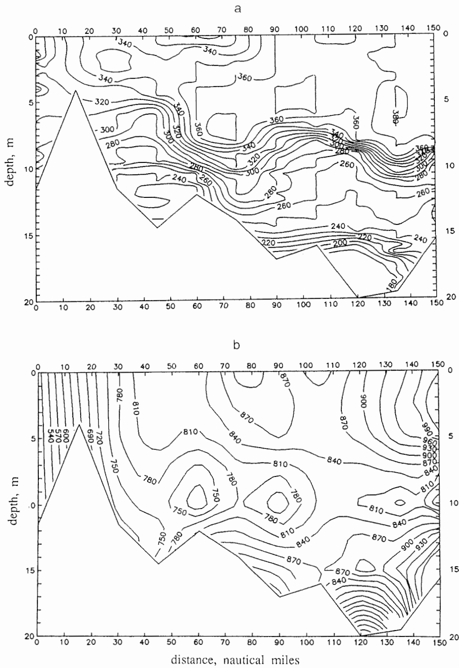
Fig. 41: (a) Fluorescence and (b) silicium distribution (mcb/l) along 134° 00' E from 74° 30' N to 72° 00' N (September 18 - 19, 1994).
