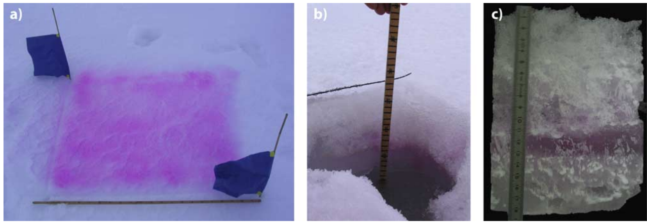
Figure 11. Photographs of tracer experiments with Sulforhodamin-B. (a) Snow surface immediately after the tracer (pink color) was sprayed homogeneously over a 1 × 1-m snow surface, marked by flags and a 1.10-m long ruler stick. (b) Snow pit 27 h after injection (for data, see Figure 12b). (c) Vertical thick section of a snow and ice sample (27 h after injection; for data, see Figure 12b). All scales are in centimeters.
