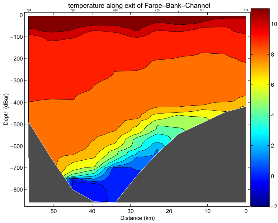
Figure 15: Potential temperature ( ^{\circ}\text{C} ) distribution of the Faroe Bank Channel exit section (FB_ex)
