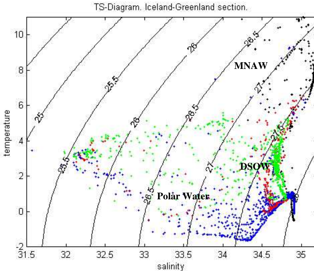
Figure 3: TS-Diagram for the main three water masses in Denmark Strait black: stations 649 - 653 blue: stations 654 - 667 red: stations 668 - 672 green: stations 673 - 683
