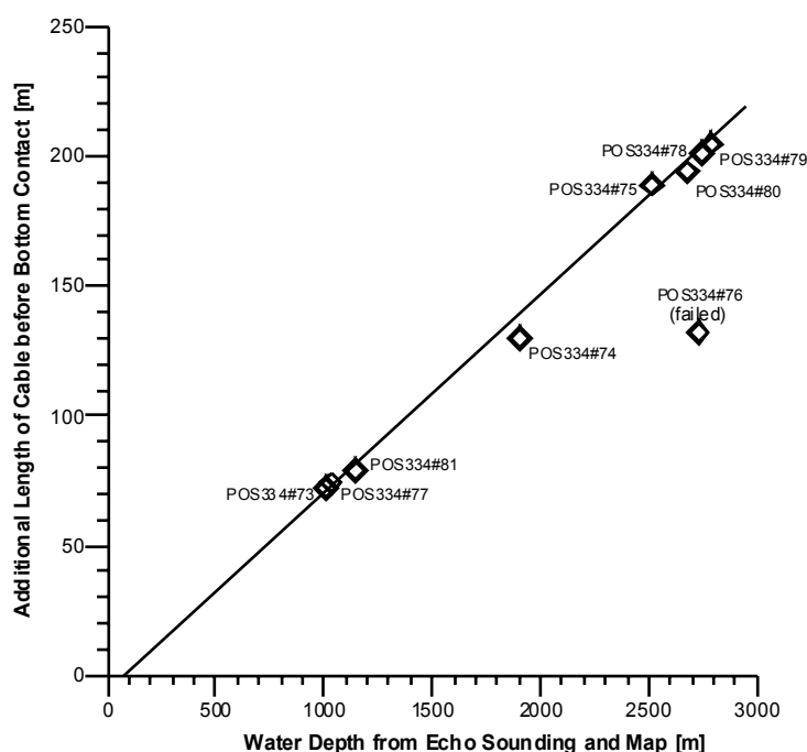
Fig. 1. Plot of the systematic offset between cable length and water depth following echo sounding at the 9 multicorer stations in the western Mediterranean.
