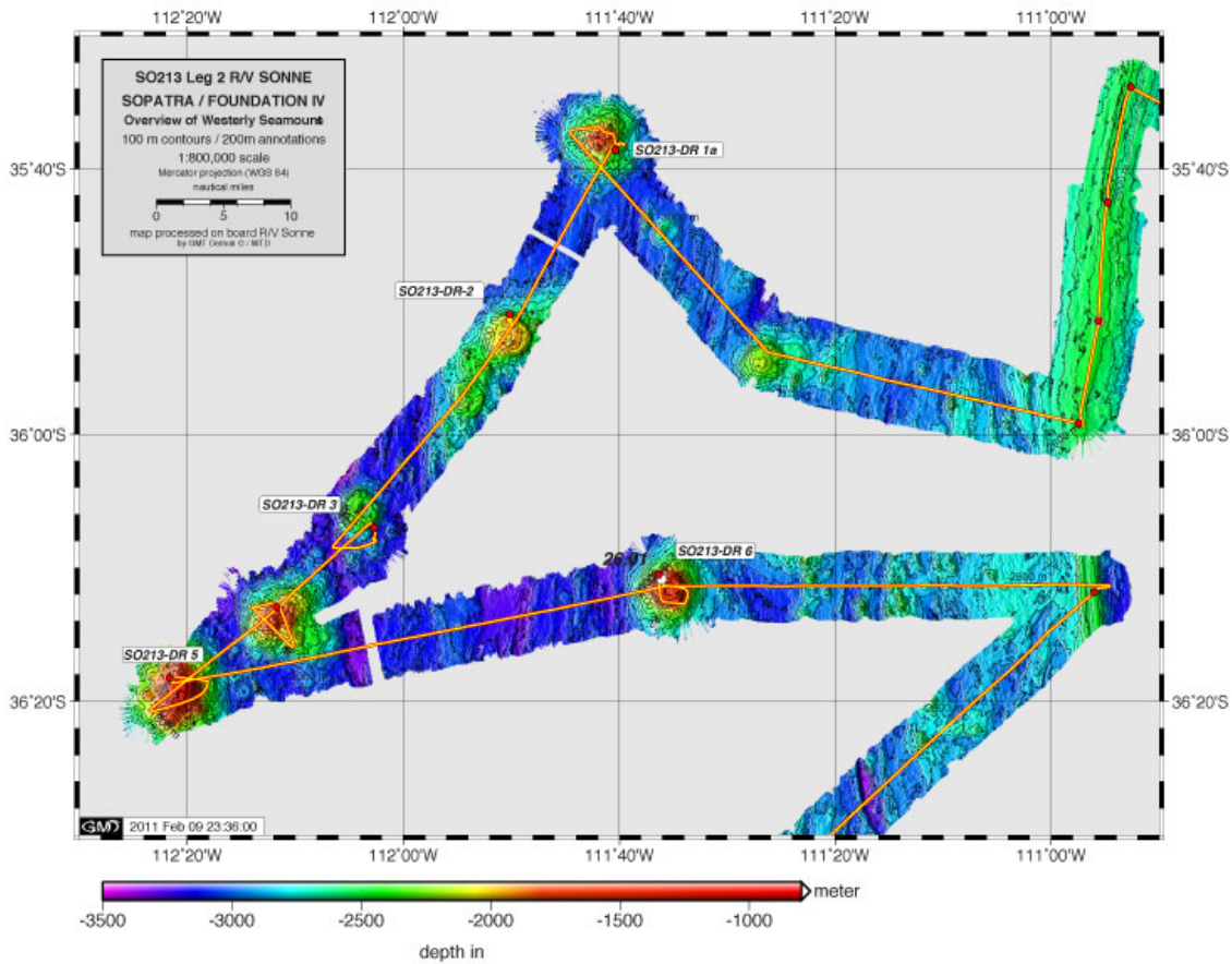
Fig. 4.9.2-3: Overview of bathymetry and dredge stations (DR) in the Westery Seamounts. Note the NE trending Westery Seamount Chain (yellow line is for ship's track). SO213 volcanology station numbers are shown only where in situ rocks were recovered. Map made with EM120 multibeam data.
