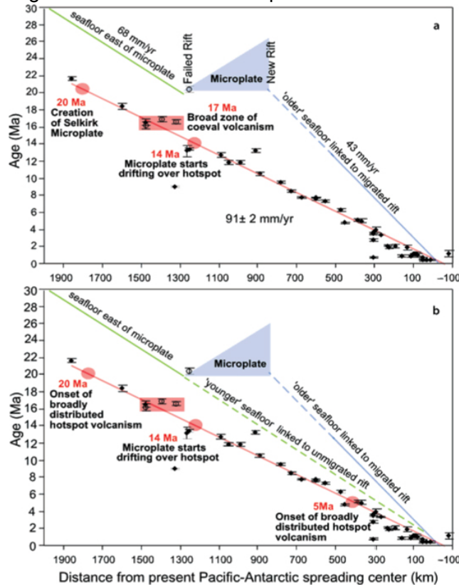
Fig. 1.4-2: (a) ^{40}\text{Ar}/^{39}\text{Ar} and older/'migrated' sea-floor age as a function of distance from the present Pacific-Antarctic spreading axis. The solid red line is the York-2 linear regression fit representing an average rate for the migration of volcanism along the chain of 91 \pm 2 \text{ mm yr}^{-1} . As the Selkirk Microplate reached the active hotspot region at about 14 Ma, much older seafloor ( \geq 6 \text{ Myr} ) began to cap the Foundation melting anomaly. This 'older'/'migrated' seafloor placed a sufficiently thick lid over most of the region impacted by the melting anomaly (pulsed plume?) to prevent the migration of hotspot melts to the seafloor during the interval ~14 Ma to ~11 Ma, resulting in the transition from broad zones of hotspot volcanism to a narrow chain of seamounts. Blue solid lines denote 'older' seafloor, unbroken blue lines indicate known sea-floor ages (Mammerickx 1992; Lonsdale 1994), and dashed blue lines indicate extrapolated sea-floor ages. The red swath indicates the broad zone of scattered coeval hotspot volcanism (open spheres) created by the proposed 17 Ma pulse of the Foundation plume crosscutting the narrow Foundation Chain. Analytical error bars are \pm 2\sigma . (b) Younger/ 'unmigrated' sea-floor age as a function of distance from the present Pacific-Antarctic spreading center – other details are the same as in Part a. The long green dashed line indicates younger/'unmigrated' sea floor created by the spreading center north of the 'Failed Rift'. The spreading center north of the 'Failed Rift' probably continued spreading normally so that 'younger' ( \leq 6 \text{ Ma} ) seafloor could move over the northern flank of the Foundation hotspot. This younger/'unmigrated' seafloor drifting by the northern flank of the Foundation melting anomaly was thin enough to allow the passage of melts along a narrow strip leading to the creation of a correspondingly narrow chain of Foundation Seamounts.
