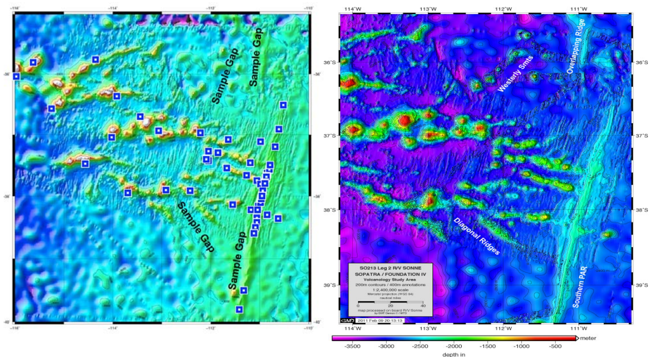
Fig. 1.4-5 (left): GEBCO 8 map of the intersection region of the Foundation Chain and the PAR show existing dredge samples and sampling gaps that are the focus of the SO213 volcanology project.
