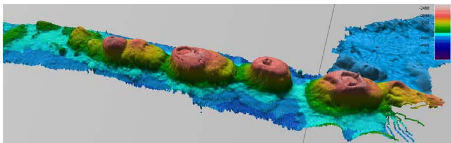
Fig. 4.5.2-2: Seamount chain in Fledermaus 7.2 (unprocessed data)
