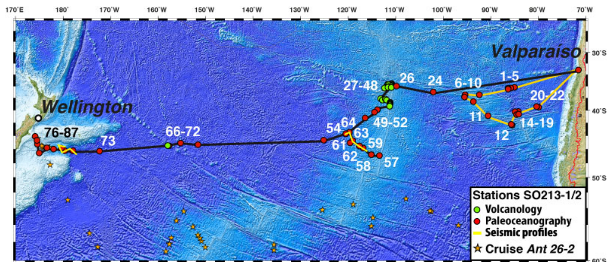
Fig. 4.6-1B: Cruise track with all station stations during Sonne expedition SO213. Paleoceanographic stations are marked by red dots.
