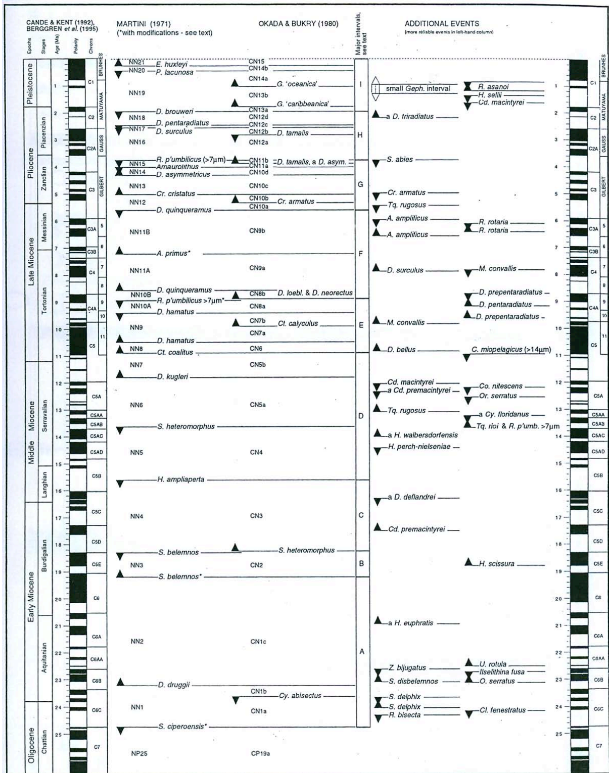
Fig. 4.7.3-3. Summary of Neogene nannofossil biostratigraphic zonation schemes and bioevents (Bown, 1998) used for this report (a=acme).
