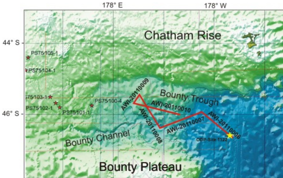
Fig. 4.8.2-5: Bathymetric map of the Bounty Trough east off New Zealand. Thick red lines mark the location of the seismic reflection profiles AWI-20110006 to AWI-201100010. Thin red lines show former tracks. Stars mark the location of Sediment cores of RV Polarstern cruises (red) and the ODP Site 1122 (yellow).
