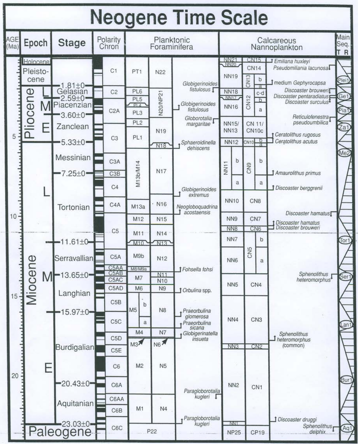
Fig. 4.7.3-2. Neogene Time Scale used for this report (Lourens et al., 2004). It includes stratigraphic subdivisions, geomagnetic polarity scale, and selected datums of planktonic foraminifera and calcareous nannoplankton.
