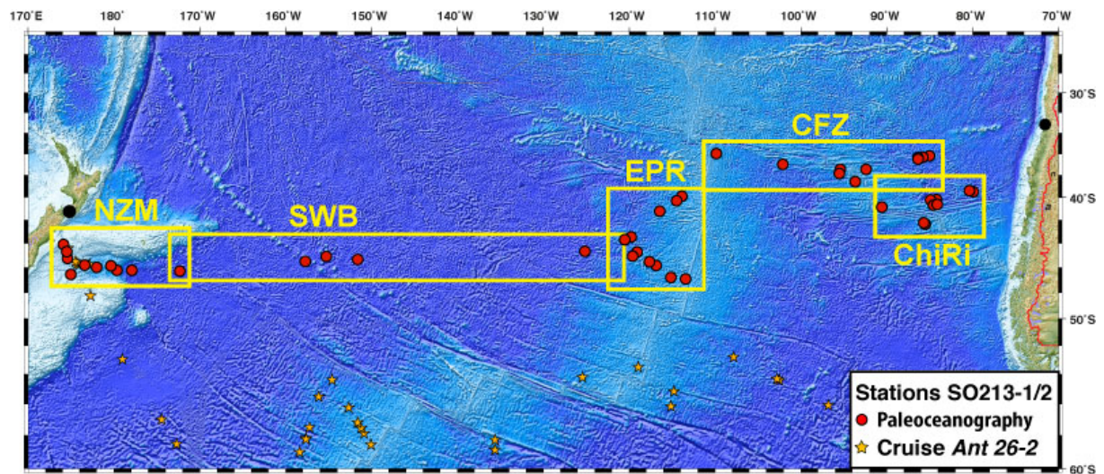
Fig. 4.6-1A: Overview map with working areas and coring stations during Sonne expedition SO213 (red dots) and Polarstern expedition ANT26-2 (yellow stars).
