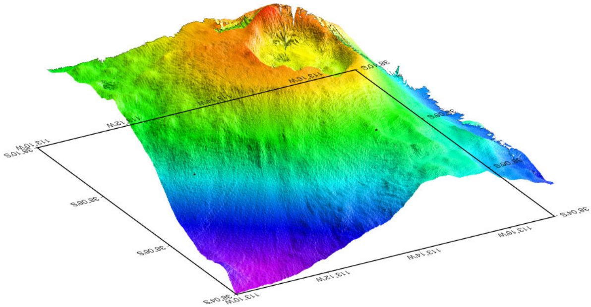
Fig. 4.9.2-11: Three-dimensional map shown caldera structure on seamount at the NW end of Diagonal Ridge #1. See Figure 4.9-9 for location of DR 7a on this volcano. Map made with EM120 multibeam data.
