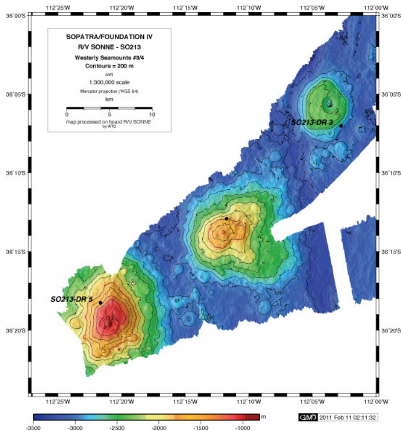
Fig. 4.9.2-5: Dredge station DR 2 on the second volcano sampled in the Westery Seamount Chain (see Fig. 4.9.2-3). Note small caldera on the top. Map made with EM120 multibeam data.
