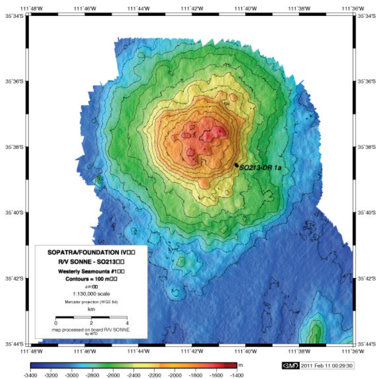
Fig. 4.9.2-4: Dredge station DR 1a on the seamount at the northern end of the Westery Seamount Chain (see Fig. 4.9.2-3). Map made with EM120 multibeam data.
