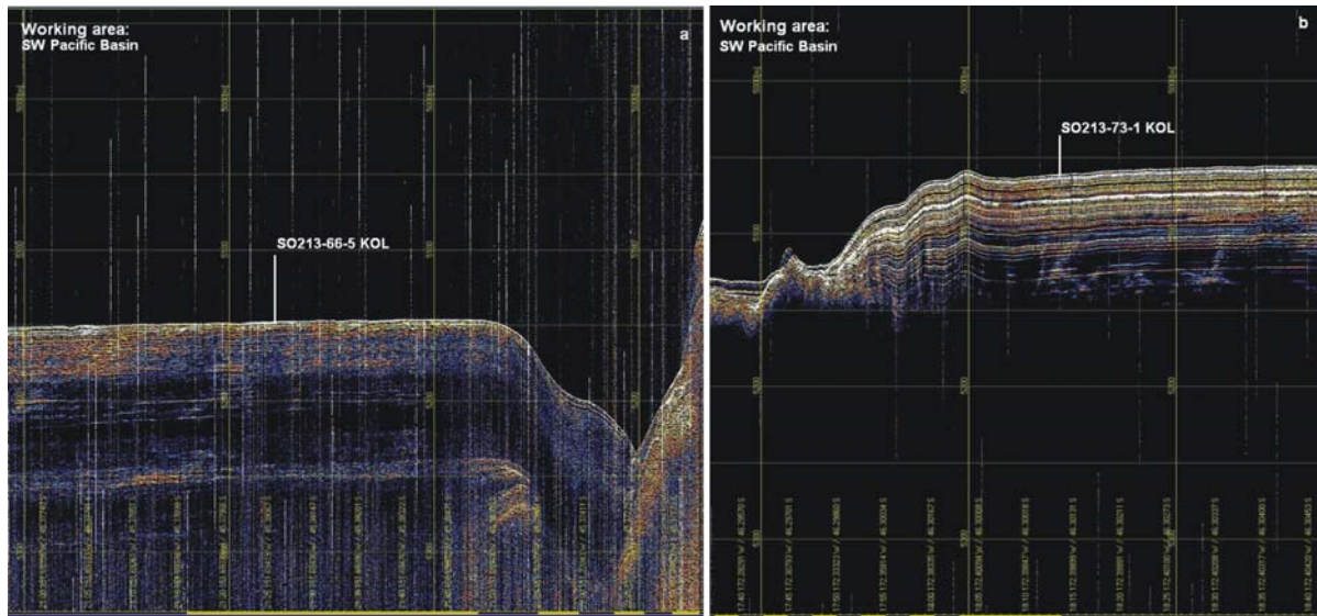
Fig. 4.5.4-4a-b: Summary of selected PARASOUND profiles with coring sites (vertical white bars) in the SW Pacific Basin
