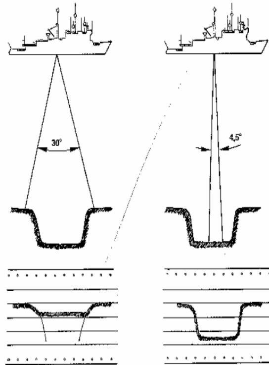
Fig. 4.5.3-1: The extremely narrowed beam of 4.5° of the ATLAS PARASOUND compared to a conventional echosounder system with an angle of 30°. The ATLAS PARASOUND even resolves small-scale bottom structures and offers a deeper penetration into the seafloor (ATLAS Hydrographic).
