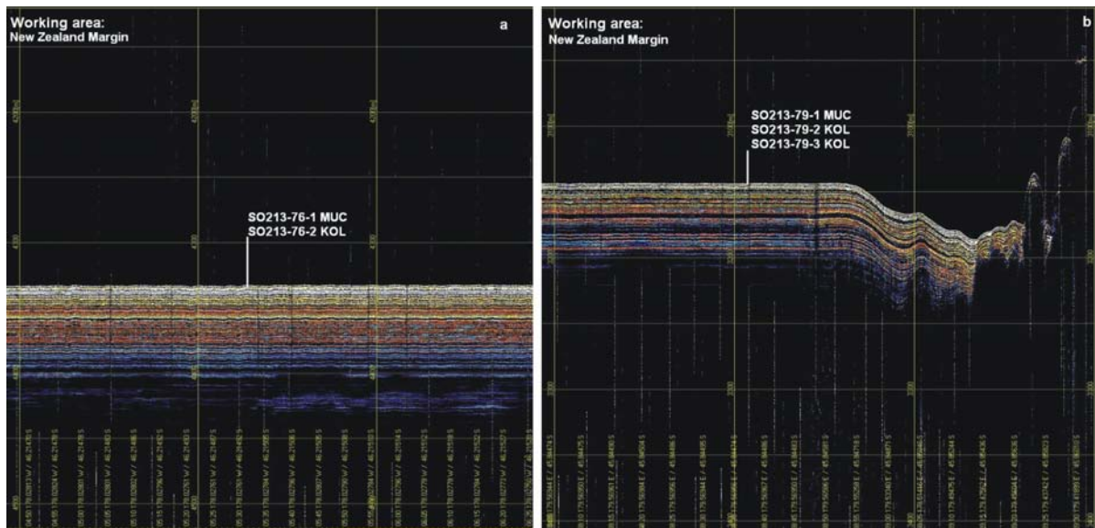
Fig. 4.5.4-5a-b: Summary of selected PARASOUND profiles with coring sites (vertical white bars) at the New Zealand Margin. Please note the well-defined sediment horizons.
