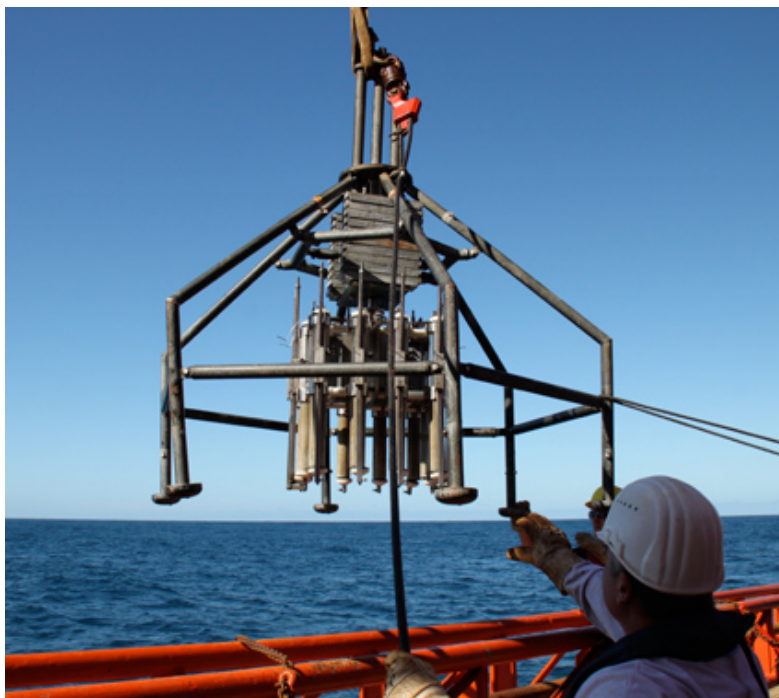
Fig. 4.6.1.-1 AWI multicorer, technical specifications:
