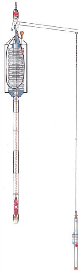
Fig. 4.6.2-1. Operation of a 15 m piston corer during SO213-1 (right) and schematic diagram of the split-piston corer from Fa. Marinetechnik Kawohl, deployed during SO-213-1
