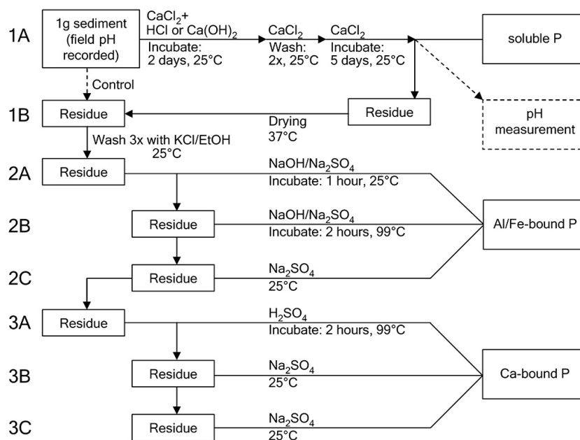
Figure 3. CONVEX scheme for the quantification of phosphorus species in sediment. 1A/1B: conversion procedure, 2A–3C: extraction procedure. For addition experiments, reference minerals were added to the sediment subsamples before incubation. Adapted from Oxmann et al. (2008).
