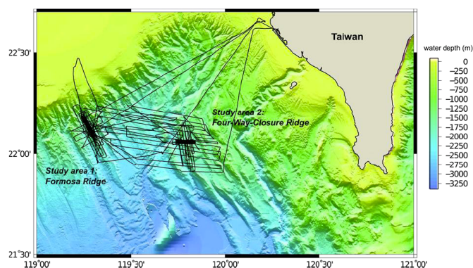
Fig. 1: Bathymetric map with cruise track of the German RV Sonne (SO227, 2.4.2013 Kaohsiung – 2.5.2013 Kaohsiung). Geophysical experiments to image fluid flow and methane hydrates have been carried out in two target areas representing an passive erosional setting (Formosa Ridge) and active accretionary setting (Four-Way-Closure).
