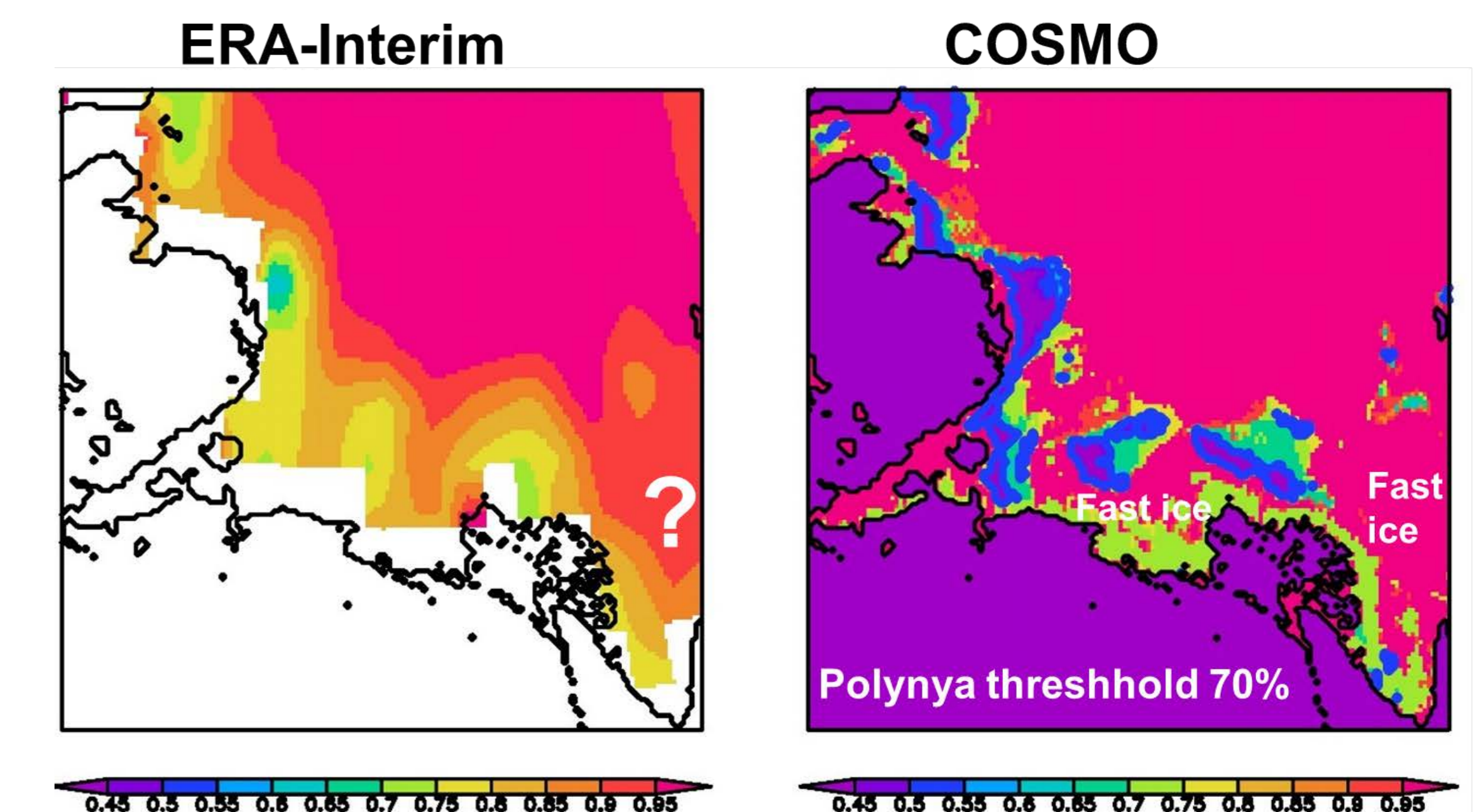
Fig.5: Sea ice concentration for 8 Jan 2009. Left: ERA-I; right: COSMO. A threshold of 70% is used in COSMO to define the polynya area. In ERA-I, fast ice areas are incorrectly represented as areas with ice concentration of 75-90%, and polynyas are smoothed out.
