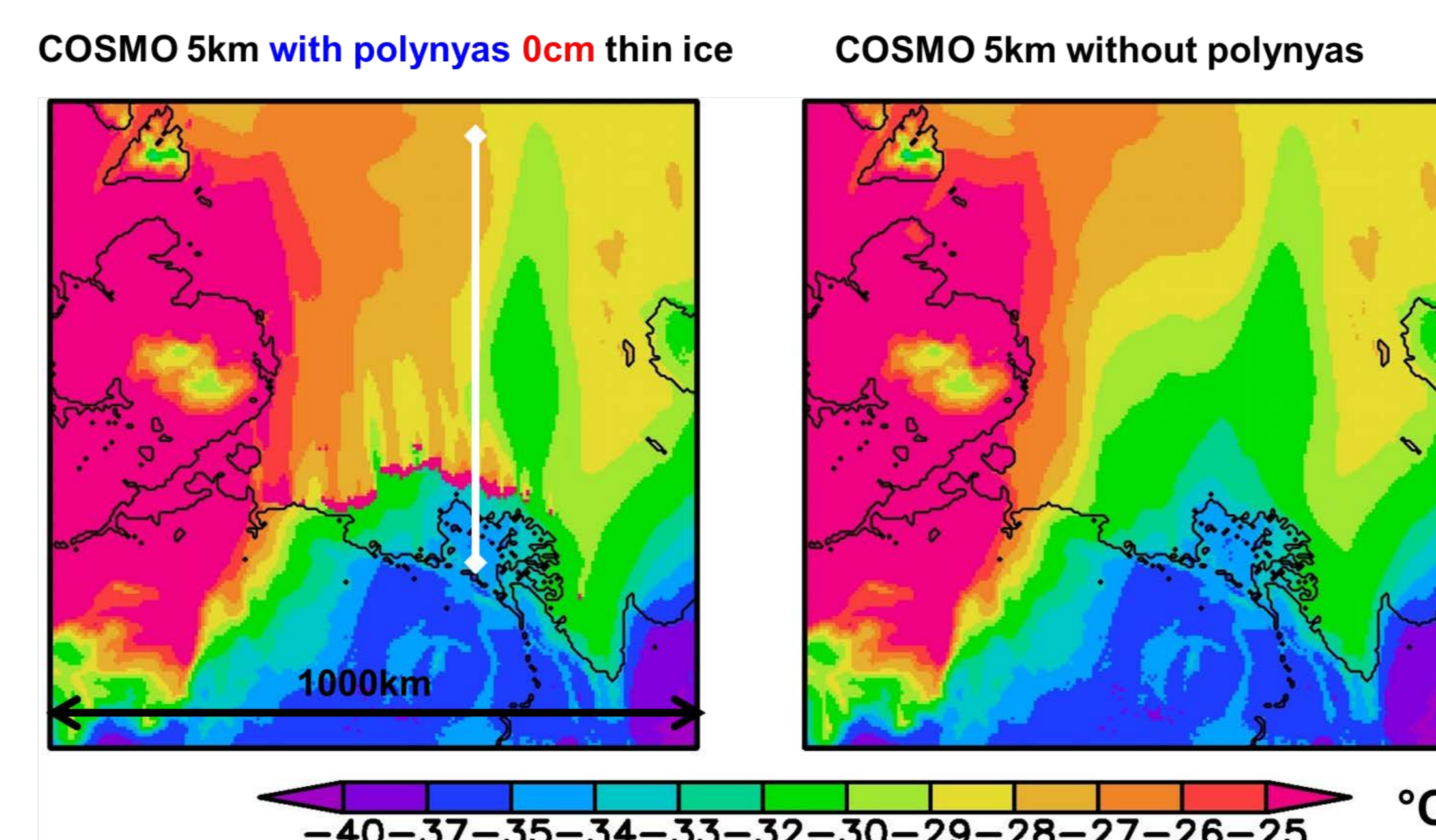
Fig.3: 2m temperature for 0700UTC 4 Jan 2008 (COSMO forced by GME). Left: open water polynyas; right: run without polynya. The white line marks a cross-section.
