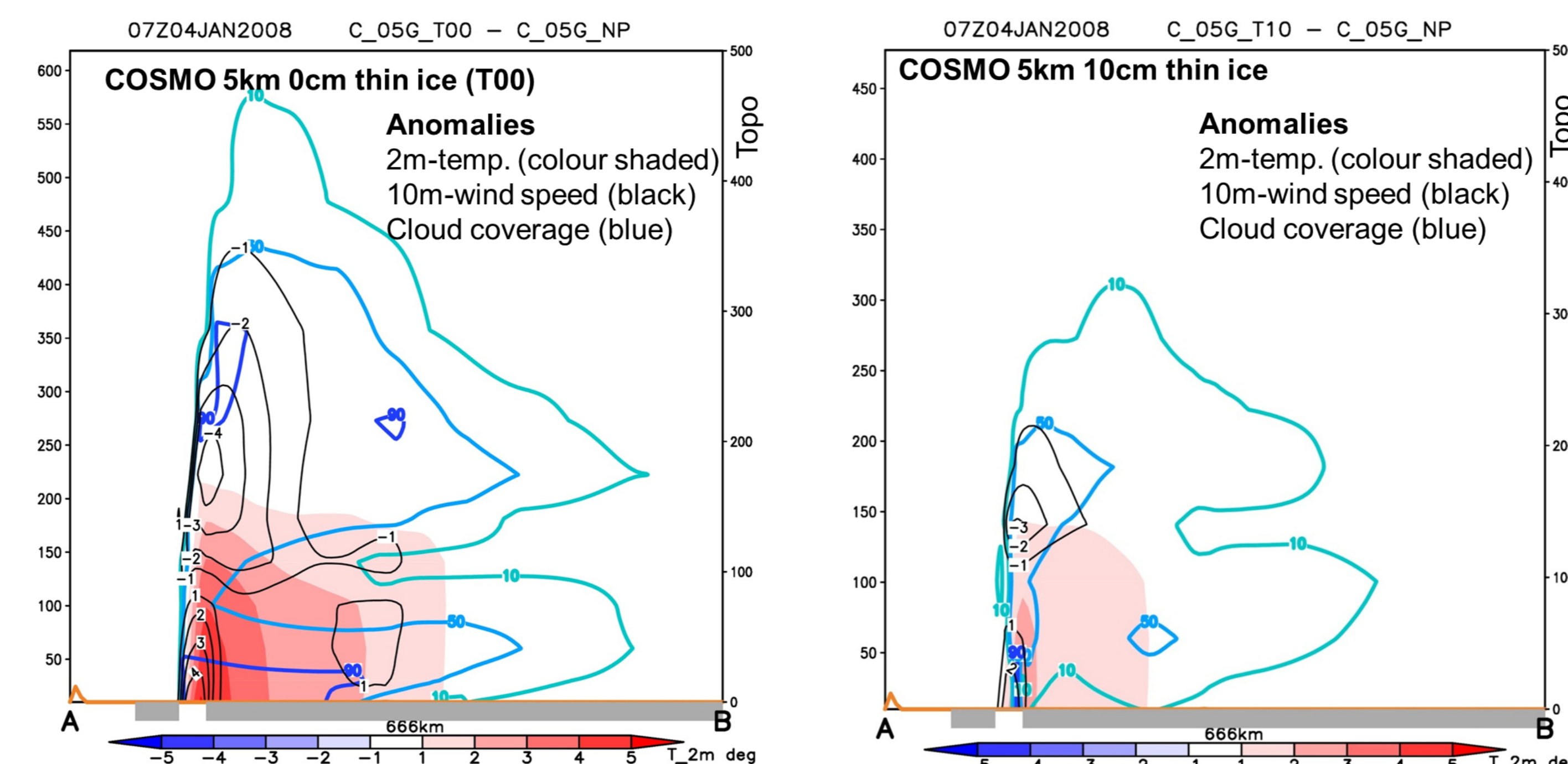
Fig.4: Cross-section along the line marked in Fig.3 for differences between the runs with and without polynyas: temperature (colour shaded), wind speed (black isolines every 1 m/s) and cloud coverage (colour isolines 10, 50, 90%). Left: open water polynya, right: polynya with 10cm thin ice.
