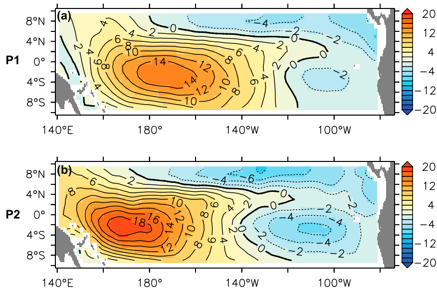
FIG. 7. Ensemble mean from the eight reanalysis products of zonal wind stress anomalies ( 10^{-3} \text{ N m}^{-2} \text{ K}^{-1} ) for (a) P1 and (b) P2.
