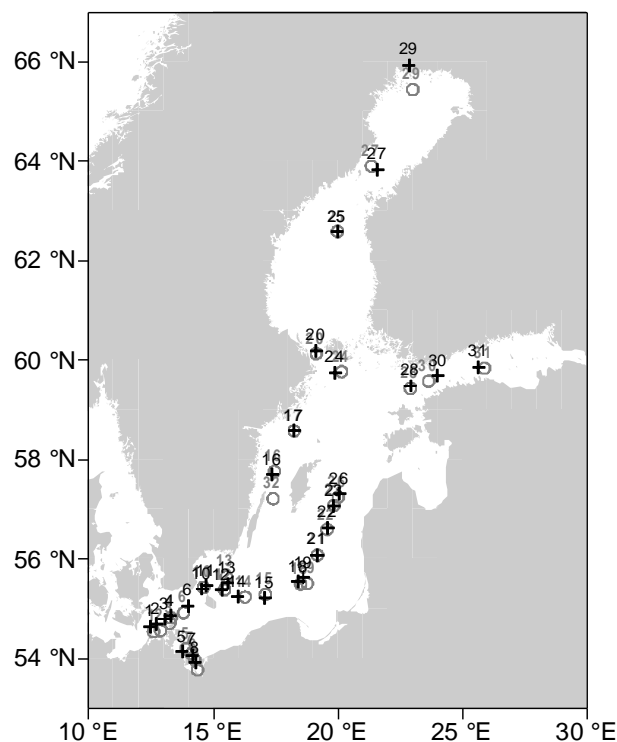
Figure 4. Station map for the comparison of isotope patterns in the water column and sediments. Gray circles are the stations referred to in Voss et al. (2005) and black crosses are those from this study. Isotope values were compared at stations with the same number.
