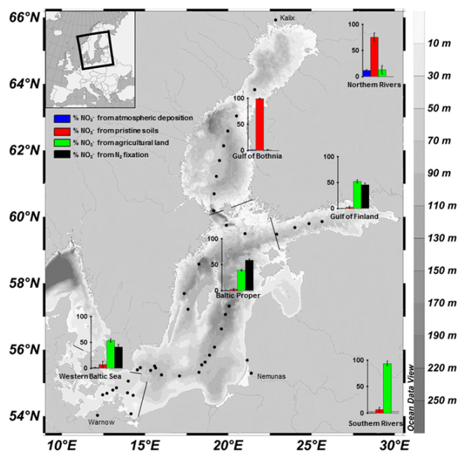
Figure 1. Station Map of the Baltic Sea and percent contribution of the four nitrate sources, \text{NO}_3^- from atmospheric deposition (blue), pristine soils (red), agricultural runoff (green), and \text{N}_2 fixation (black), for the Western Baltic Sea, Baltic Proper, Gulf of Finland, Gulf of Bothnia, southern rivers, and northern rivers. Stations are indicated as black dots. For more details see Supplement Table 1.
