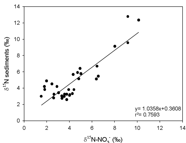
Figure 3. \delta^{15}\text{N} from sediment samples vs. \delta^{15}\text{N}-\text{NO}_3^- from surface water samples. \delta^{15}\text{N} values from sediments were taken from Voss et al. (2005). The positive slope suggests a tight coupling between \delta^{15}\text{N}-\text{NO}_3^- in surface waters and \delta^{15}\text{N} in sediment samples.
