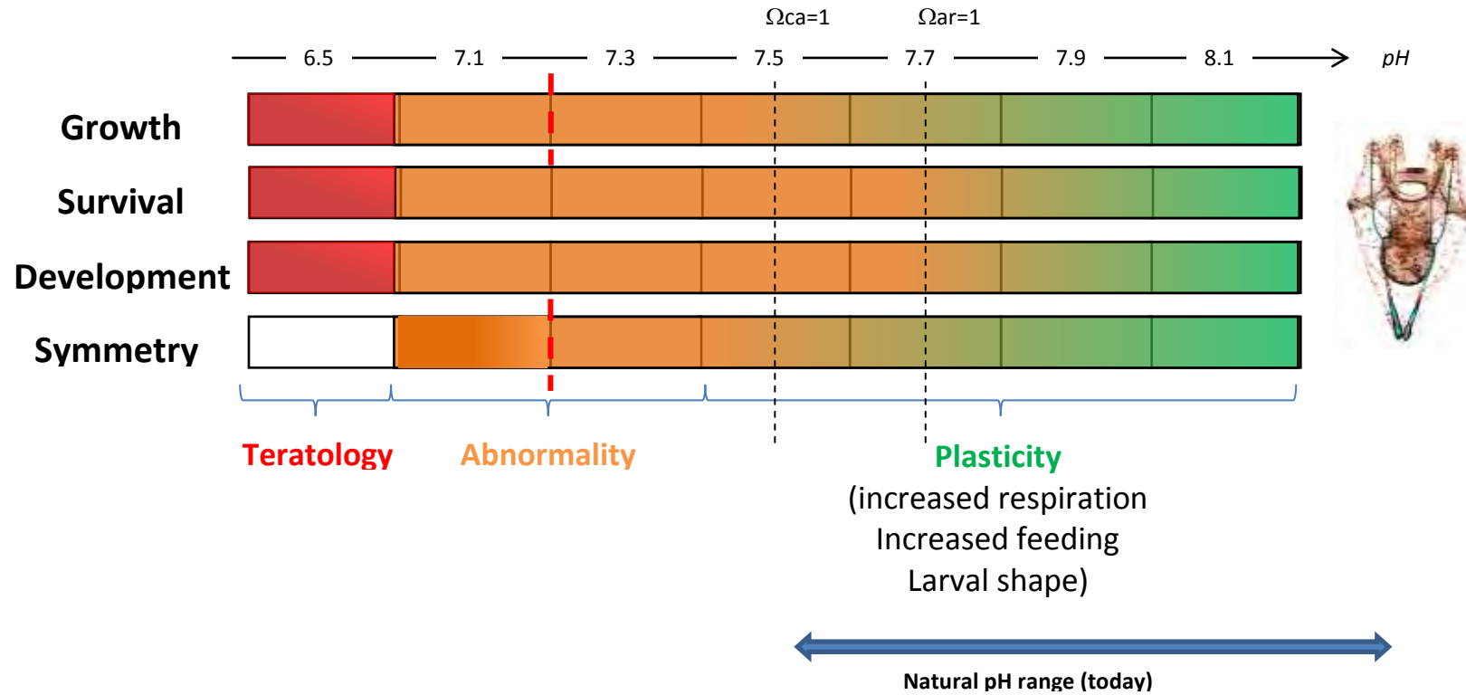
Figure 24. Synthesis of the work of Chan et al. 2012; Dorey et al. 2013; Stumpp et al. 2012 summarising the impacts of elevated pCO_2 on larval biology using the urchins Strongylocentrotus droebachiensis and S. purpuratus as models. In general, larvae are found to be more susceptible than adults to elevated pCO_2 /reduced pH but that different sub-lethal effects are produced at different pH tipping points.
