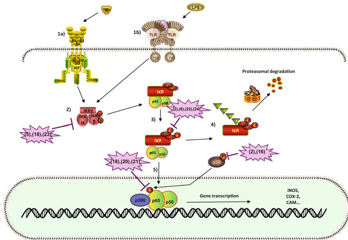
Fig. 4 Involvement of naturally occurring chalcone derivatives in the NF- \kappa B inflammation pathway. 1a TNF \alpha and/or 1b LPS ligands interact with corresponding receptors, recruiting several signaling proteins to form a primary signaling complex. 2 Transmission of signal resulting in IKK activation. 3 IKK subsequently phosphorylates serines 32 and 36 of the I \kappa B inhibitor, 4 which in turn creates binding sites for ubiquitination and shifts I \kappa B to proteasomal degradation. 5 NF- \kappa B subunits are released from the inhibitor complex and translocated to the nucleus where they bind DNA and activate transcription of several genes. Chalcone derivatives block the NF- \kappa B
