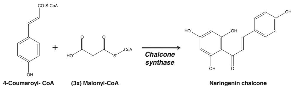
Fig. 2 Biosynthesis of naringenin chalcone in plants and citrus. The condensation of three molecules of malonyl-CoA and one molecule of 4-coumaroyl-CoA is catalyzed by chalcone synthetase
