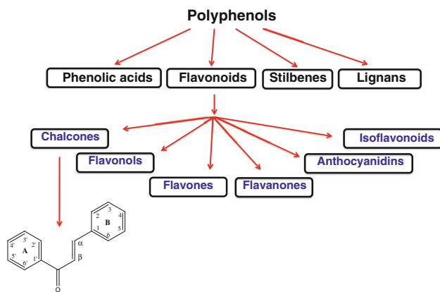
Fig. 1 Schematic representation of main polyphenol family members. Polyphenols are subdivided into 4 main classes—phenolic acids, flavonoids, stilbenes, and lignans—according to the number of phenol rings they include and the structural elements that bind these rings together [114]. Flavonoids can be further divided into various subclasses of which chalcones, flavonols, flavones, flavanones, anthocyanidins, and isoflavonoids are the most common. The core 1,3-diphenyl-2-propenone chalcone structure is shown
