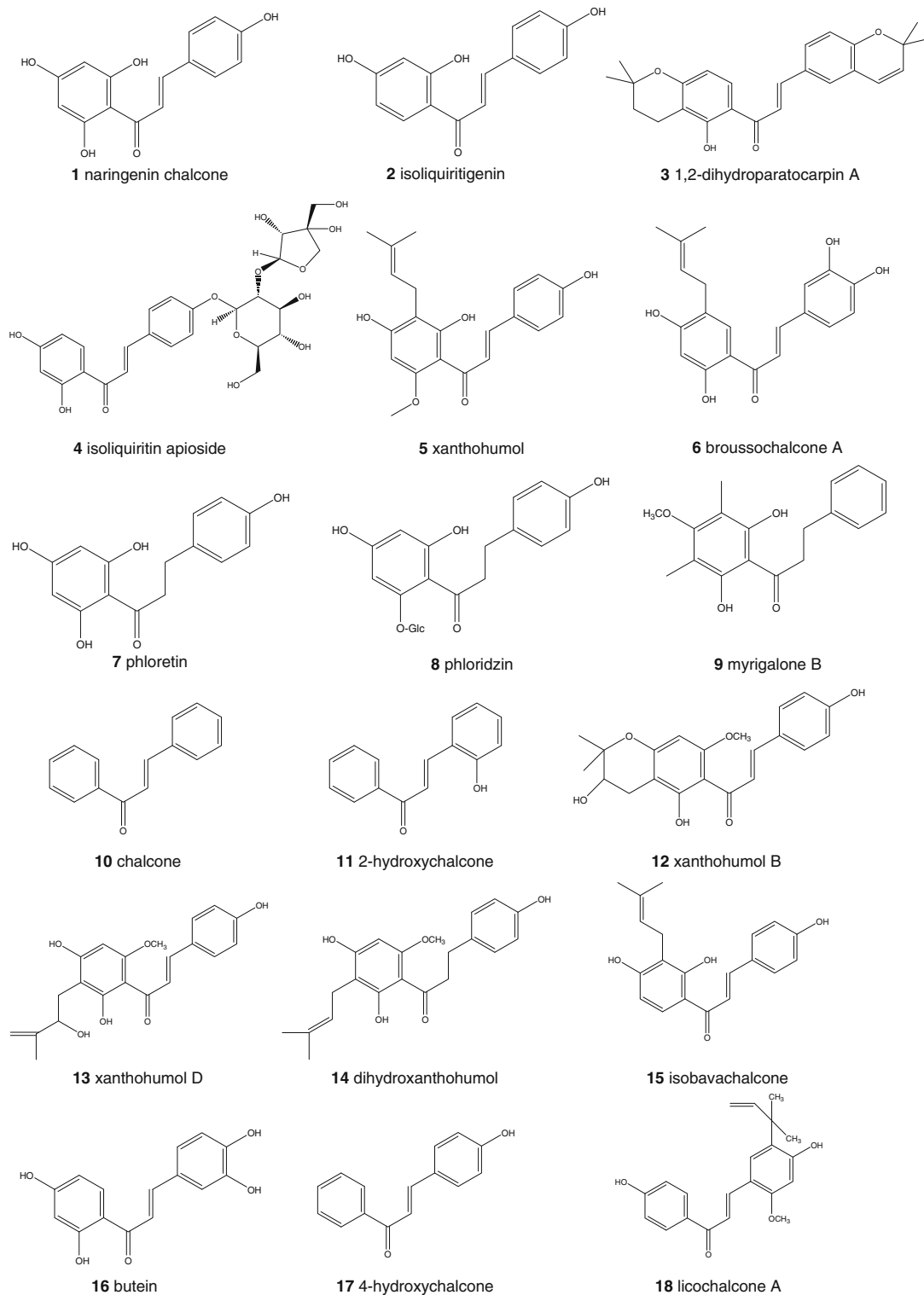
Fig. 3 Chemical structures of naturally occurring chalcone derivatives
