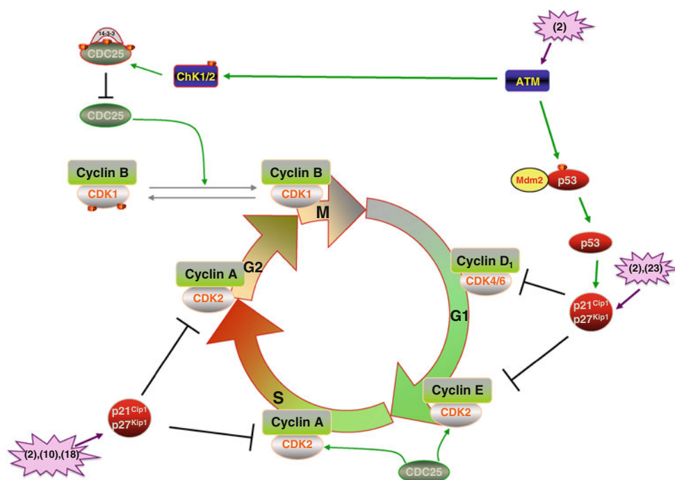
Fig. 5 Involvement of naturally occurring chalcone derivatives in regulation of the cell cycle. Chalcone derivatives may induce ATM (chalcone 2 ), which in turn phosphorylates p53, thus decreasing p53/MDM2 interaction. However, ATM augmentation subsequently leads to phosphorylation of Chk1 and Chk2 and reduces the level of Cdc25c resulting in G2/M arrest. By activating inhibitors of Cdks (p21 and p27), chalcone derivatives may participate in cell cycle arrest in either
