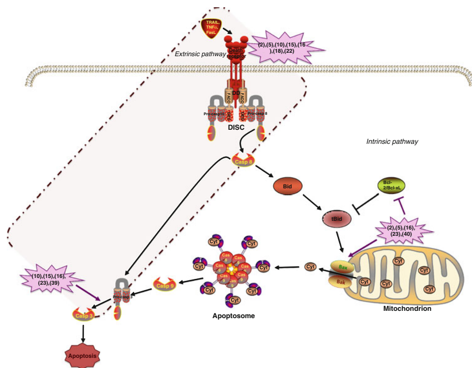
Fig. 6 Involvement of naturally occurring chalcone derivatives in apoptotic cell death. Chalcones potentiate the extrinsic apoptotic pathway: chalcones enhance the apoptosis-inducing potential of TRAIL partially by increased expression of death receptors DR4 and DR5 (chalcones 2 , 5 , 10 , 15 , 16 , 18 , 22 ). Chalcones are implicated in the intrinsic apoptotic pathway: chalcones target mitochondria either by disruption of the mitochondrial membrane potential (chalcones 2 , 5 ) or by downregulation of anti-apoptotic proteins like Bcl-xL, Bcl-2, and upregulation of Bax and Bak (chalcones 16 , 23 , 40 ). Chalcones
