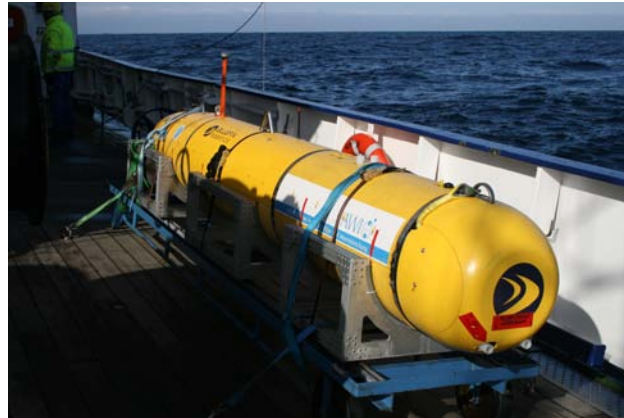
Fig. 5.3.1: AUV (AWI) for water column studies above the seafloor
