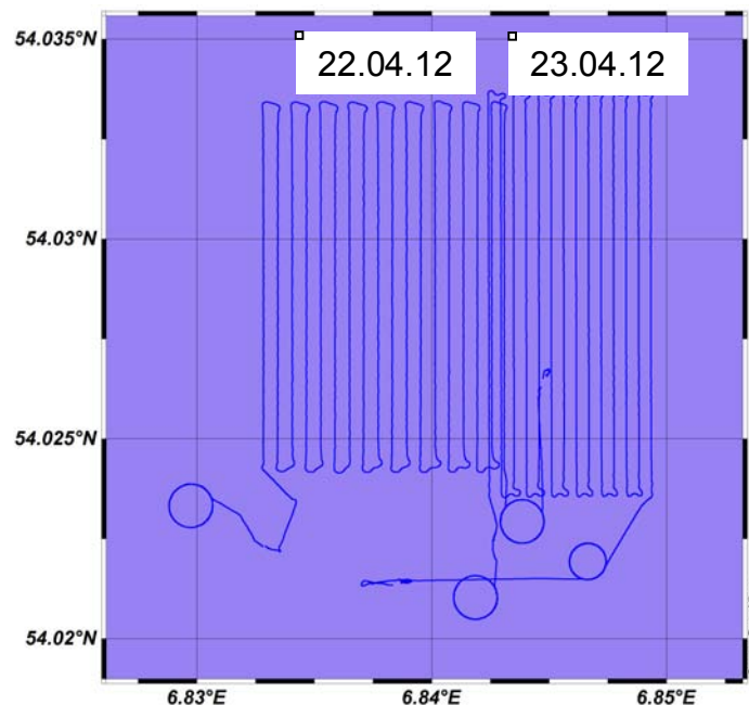
Fig. 5.3.2: AUV search grids during HE-377
