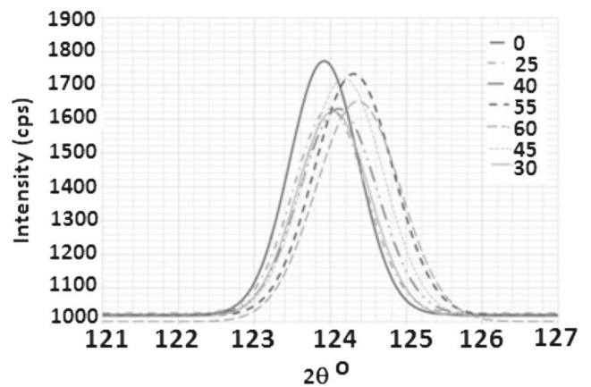
Fig. 4 Evolution of the diffraction angle 2\theta depending on the angles \psi for the G10380 burnished samples with vibration
