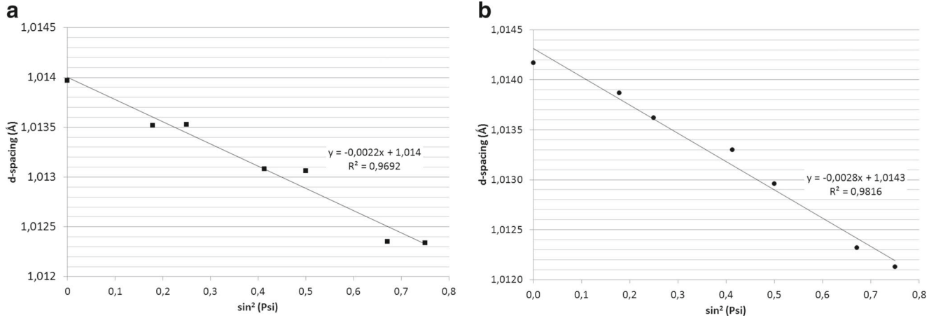
Fig. 5 Evolution of d-spacing based on \sin^2\psi for the burnished G10380 samples. a NVABB. b VABB
