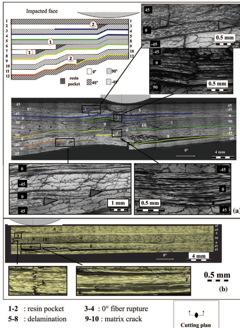
Fig. 6. Micrograph of (a) – A_5^t specimen, (b) – A_6^* specimen [26]. (For interpretation of the references to colour in this figure legend, the reader is referred to the web version of this article.)
