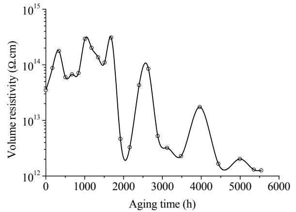
Fig. 5. Volume resistivity evolution versus aging time.
