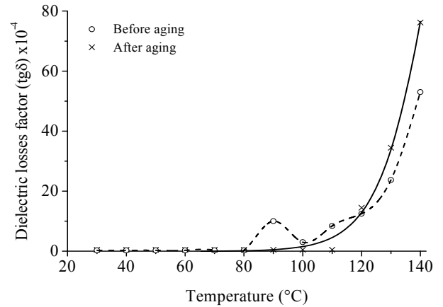
Fig. 2. Temperature dependence of dielectric losses factor before and after wet aging.
