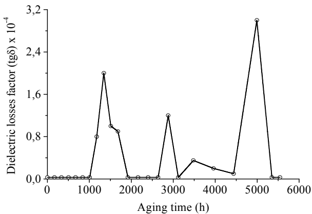
Fig. 1. Dielectric losses factor variations with respect to aging time.
