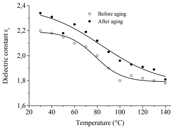
Fig. 4. Temperature dependence of dielectric constant before and after moisture exposure.
