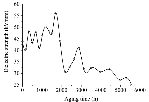
Fig. 6. Dielectric strength changes versus aging time.
