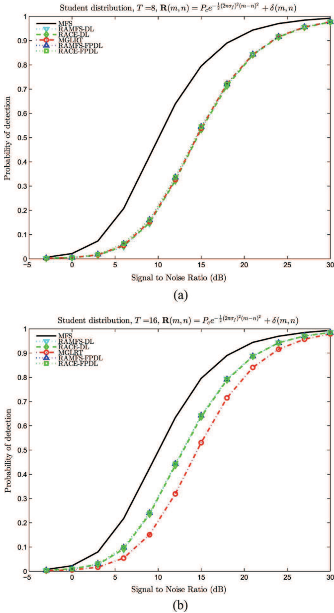
Fig. 1. Probability of detection of the various detectors versus SNR . (a) T = 8 , (b) T = 16 .
