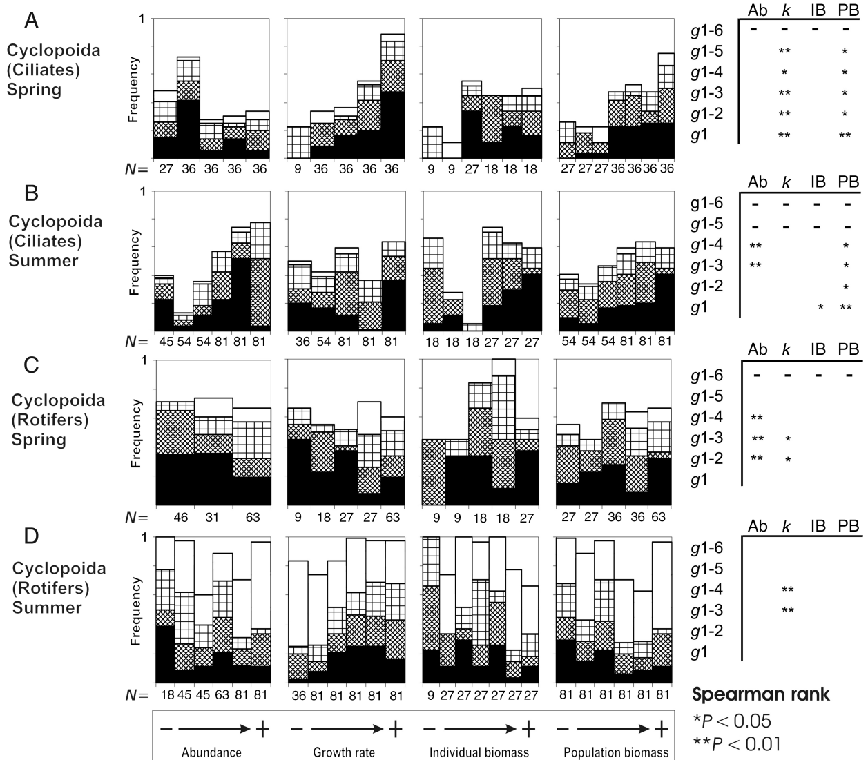
Fig. 4. Cumulated frequencies of the predation rate ( g ) ranks of Cyclopoida on ciliates [(A) spring and (B) summer] and on rotifers [(C) spring and (D) summer] in relation to the abundance (Ab) rank, the growth rate ( k ) rank, the individual biomass (IB) rank and the population biomass (PB) rank of the prey. The black, cross-hatched and squared bars are the first, second and third g -ranks. The white bars are the fourth and more g -ranks. The white area above the bars represents the frequency of the negative or zero g . N is the number of occurrences used for the calculation of the frequencies. Significant positive correlations between g frequencies and an increase/decrease in the prey characteristics frequencies are shown on the right. Spearman rank correlation was applied to each of the cumulative series of the positive g ranks, from the first g -rank ( g_1 ) to the sixth g -rank ( g_6 ); the minus sign indicates the absence of cumulative series and significances are shown as asterisks.
