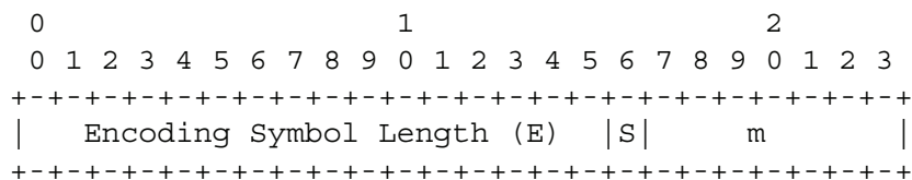
Figure 3: FSSI encoding format.
