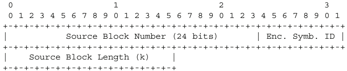
Figure 5: Source FEC Payload ID encoding format for m = 8 (default).
