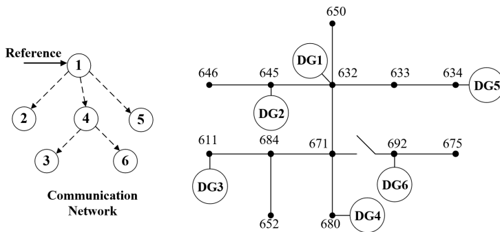
FIGURE 16 Diagram of modified IEEE-13 bus MG system
