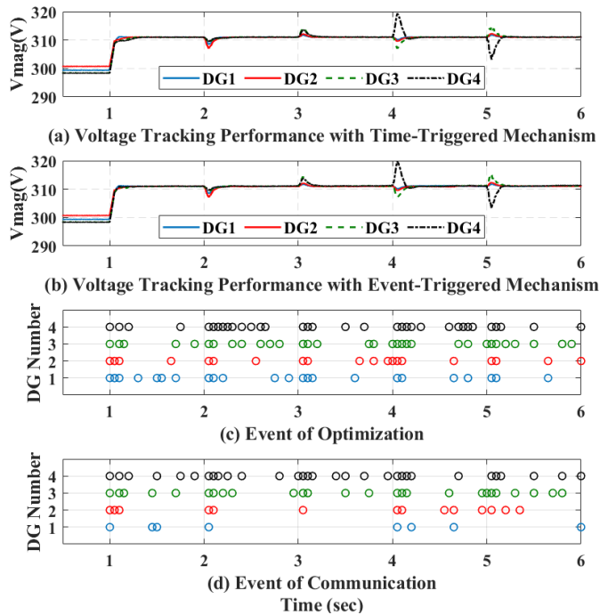
FIGURE 7 Voltage control performance by using event-triggered mechanism: (a) voltage tracking performance with time-triggered mechanism; (b) voltage tracking performance with event-triggered mechanism; (c) event-triggered time of DMPC optimization; (d) event-triggered time of neighbouring communication.
