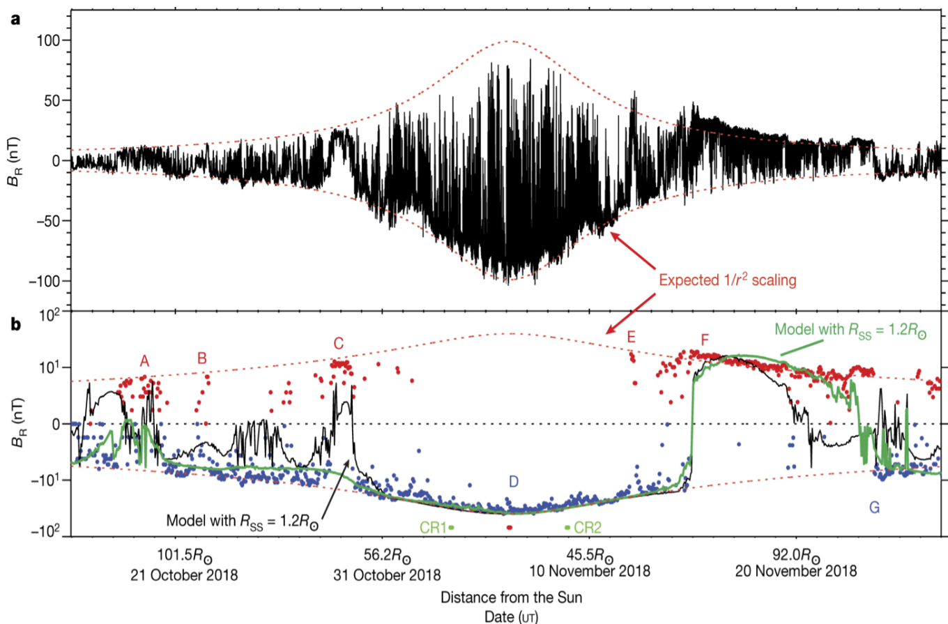
Fig. 2. (a) PSP measured radial magnetic field B_R over the first PSP encounter. The magnitude scales approximately as 1/r^2 (red dotted lines; also in Fig 4b). We highlight the rapid large-amplitude polarity reversals ( \delta B_R/|B| of the order of 1). (b) One-hour statistical modes of B_R (bisymmetric logarithmic plot) show the large-scale radial field colored for polarity (red, outward; blue, inward). Predicted radial-field profiles from a PFSS model are shown in green and black (SS at 2.0 and 1.2 RS respectively). Adapted from Bale et al. (2019) .
