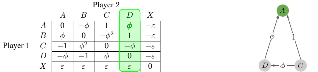
(c) The \alpha -Rank distribution over \{C, D\} puts all mass on D ; the best response against D is A .
