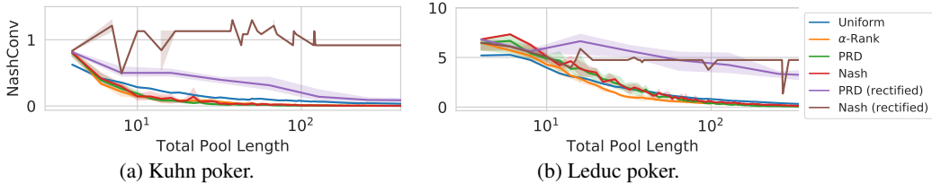
Figure 3: Results for 2-player poker domains.
