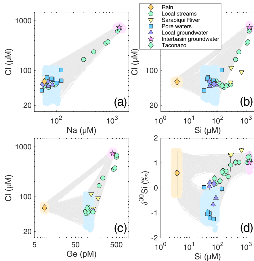
Figure 4. The range of chemical and \delta^{30}\text{Si} compositions in La Selva streams and other water samples. In each panel, the gray area shows the mixing space between rainwater, lowland weathering fluids (all pore waters and well samples), and interbasin groundwater (Guacimo Spring sample CR05, pink star). The mixing space is calculated from 1,000 Monte Carlo simulations, randomly sampling each end-member (shaded area around the measured sample compositions of the three end-members) from a range of values defined either by analytical uncertainty (for groundwater and rain water) or 2 SD of all pore water and well samples (for the local lowlands end-member). Rainwater composition is included to highlight the fact that soil pore waters inherit only negligible Si and Ge from rain. For rainwater, \delta^{30}\text{Si} was not measured; therefore, for visualization purposes, a range of values anywhere between -0.3 and 1.5\text{‰} was assigned, encompassing most measured silicate rock and seawater values (Frings et al., 2016).
