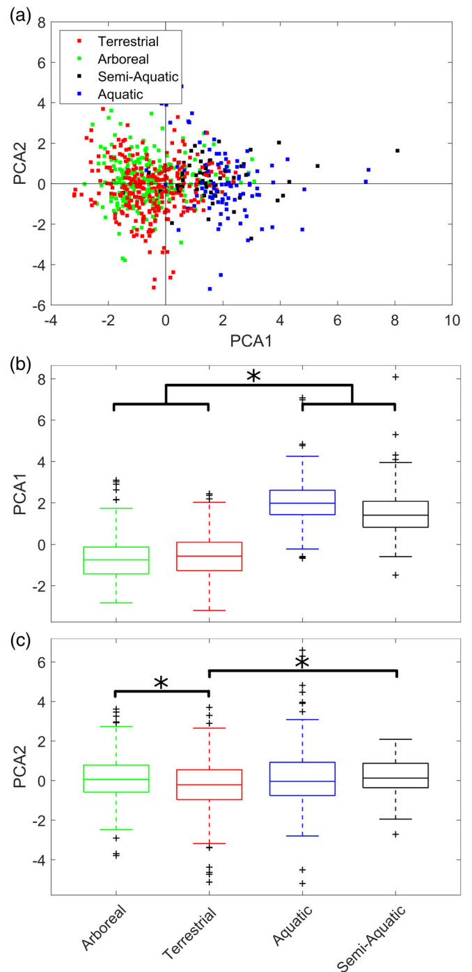
FIGURE 2 Principal component analysis (PCA) of whisker shape. (a) PC1 plotted against PC2 for all species. (b) PC1 values according to typical substrate. (c) PC2 values according to typical substrate. Black asterisks indicate significant differences. Value colours indicate typical substrate: terrestrial (red), arboreal (green), aquatic (blue) and semi-aquatic (black)
