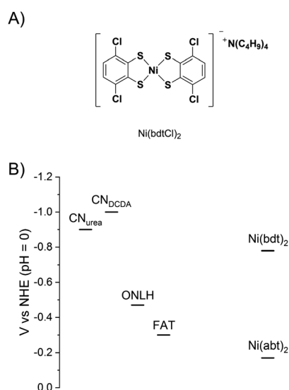
Fig. 5 (A) Structure of \text{Ni}(\text{bdtCl})_2 (B) estimated potentials of the CN conduction bands and the onset of \text{H}_2 evolution for \text{Ni}(\text{bdt})_2 and \text{Ni}(\text{abt})_2 . 3,4,26
