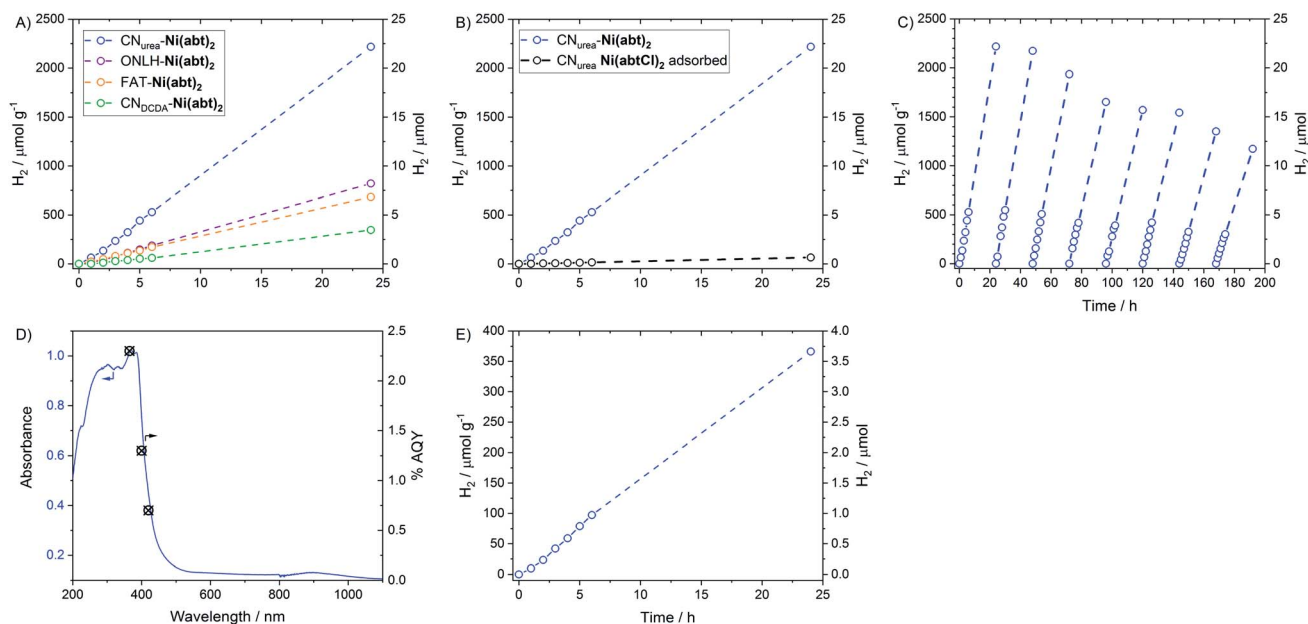
Fig. 4 Photocatalytic hydrogen production by (A) \text{CN-Ni}(\text{abt})_2 hybrids (B) \text{CN}_{\text{urea}}\text{-Ni}(\text{abt})_2 compared with \text{CN}_{\text{urea}} with \text{Ni}(\text{abtCl})_2 adsorbed (C) \text{CN}_{\text{urea}}\text{-Ni}(\text{abt})_2 activity for 8 days (D) quantum yields of \text{H}_2 overlaid with DRUVS spectrum for \text{CN}_{\text{urea}}\text{-Ni}(\text{abt})_2 . All in \text{H}_2\text{O} with 10% TEOA and \lambda > 420 nm (pH = 11). (E) ONLH- \text{Ni}(\text{abt})_2 with \lambda > 475 nm.
