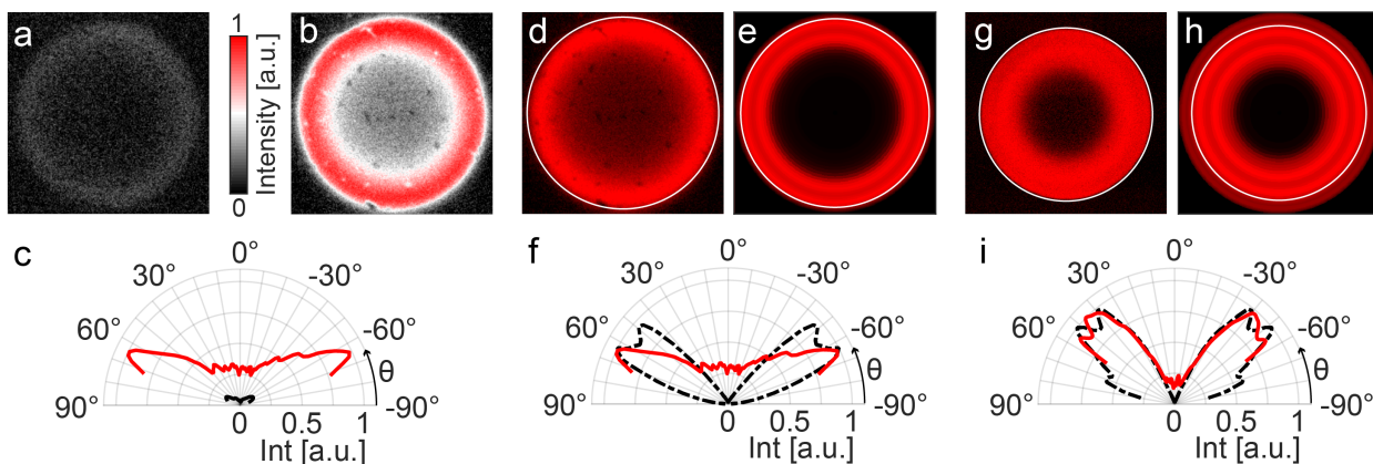
Figure 3: Optical characteristics of the light-emitting surfaces. a, b) Comparison of the emission profile of substrates with a flat bottom reflector (a) and micro-patterned reflecting bottom surface (b). c) Polar plot comparing the two specimens' angular emission profile extracted as an average of radial emission patterns from (a) and (b). The red and black curves represent data from the samples with patterned and flat bottom reflectors, respectively. d) Experimentally determined emission profile for a sample with patterned bottom reflector in air imaged with a
