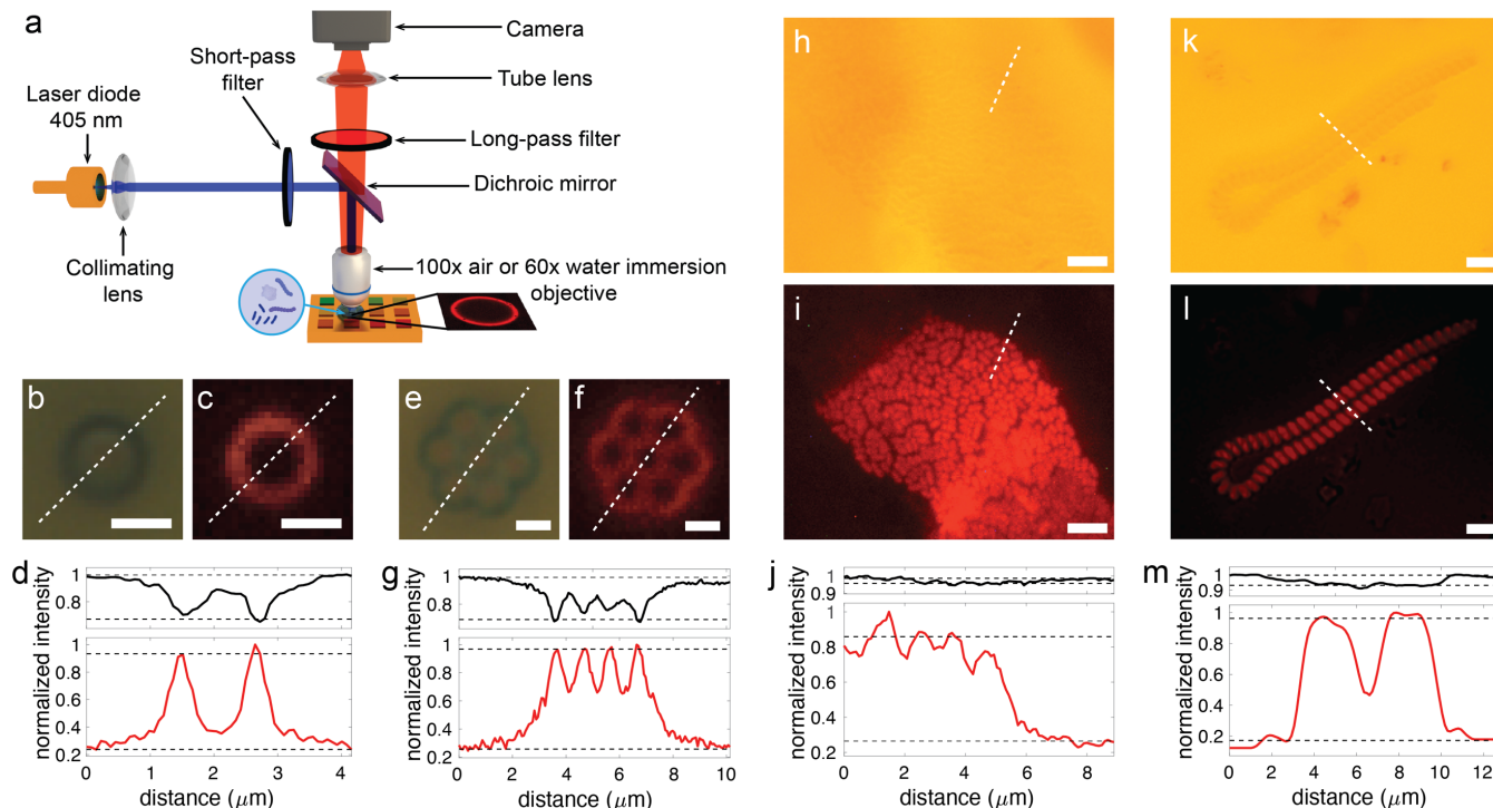
Figure 4: Application of the SLED surfaces to image colloids and marine micro-organisms. a) Schematics of the optical setup used for imaging. In the case of biological samples, a drop of water containing the micro-organisms is deposited on the SLED surface and imaged using an immersion lens. SLED measurements rely on exposure of the substrate with blue light from a laser diode. Bright-field images and SLED images together with corresponding intensity profiles (black lines – bright-field, red lines – SLED) extracted along the white dashed lines are shown in b-d) for a single colloid, e-g) for a colloid cluster, h-j) for a colony of E. coli bacteria in water, and k-m) for micro-algae in sea water. Scale bars: 1 \mu m (c, d, e, f), 5 \mu m (h, i), 10 \mu m (k, l). The dashed black lines in (d), (g), (j), and (m) indicate the levels used to determine the image contrasts specified in the main text.
