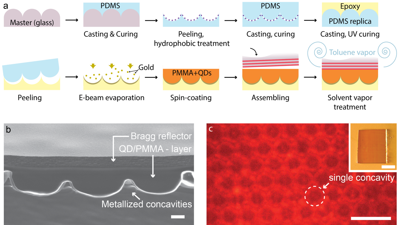
Figure 2: The fabricated SLED surface. a) Schematic of the manufacturing procedure. The patterned epoxy substrate was obtained by a three-step replica moulding procedure, consisting in casting PDMS on a glass master, PDMS casting on PDMS, and epoxy casting on the PDMS replica. Then, the SLED surface was assembled by adding the metal reflector, QDs and Bragg reflector on top of the patterned epoxy. b) Cross-sectional SEM view of the SLED device showing the patterned bottom surface, the QD-doped PMMA layer and the Bragg reflector; scale bar: 1 \mu m. c) Top view of the complete device obtained by fluorescence microscopy with the microscope's focus plane on the bottom reflector; scale bar: 10 \mu m. Inset shows a macroscopic top-view of the assembled SLED surface; scale bar: 1mm.
