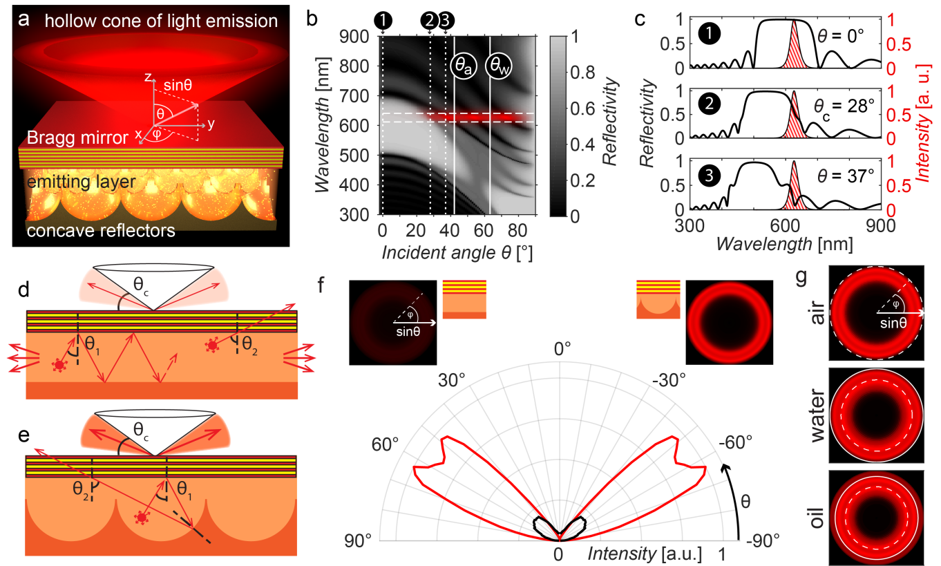
Figure 1: The concept of substrate luminescence-enabled dark-field imaging. a) 3D schematics of the device design. b) Grey-scale encoded reflectivity of a Bragg mirror with a reflection band centred at 585nm as a function of light incidence angle and wavelength. Solid white vertical lines mark the critical angles \theta_a and \theta_w beyond which total internal reflection occurs if the upper medium is air or water. The spectral emission range of the QDs is marked with horizontal dashed white lines; the red overlay represents the angle ranges at which emitted light can escape from the Bragg reflector. c) Selected spectra from (b) at incidence angles \theta = 0^\circ , \theta_c = 28^\circ (where the Bragg reflector exhibits a reflectivity of 50% for the QD's spectral emission range), and \theta = 37^\circ , marked by dotted lines in (b). The QD emission spectrum is represented as the red-hatched area. d) Schematic depicting a possible optical path of a light beam emitted by a QD in the case of a flat bottom reflector. If the light is emitted at an angle \theta_1 for which it is reflected by the Bragg mirror, the beam will keep bouncing between the two reflective surfaces, until it escapes at the sample edge. For a higher incidence angle \theta_2 light can couple out. e) In the case of a bottom reflector patterned with semi-spherical cavities, the light emitted at an angle \theta_1 can – through scattering from the patterned bottom surface – reach an incident angle \theta_2 large enough to transmit through the Bragg reflector. f) Simulated angular emission profiles comparing the angle-dependent intensity of light emitted by a substrate with flat bottom reflector (black) and a substrate with a micro-patterned bottom reflector (red). The insets show visualizations of the emitted light intensity and colour as a function of the angle of incidence onto the Bragg reflector, which increases from 0^\circ at the images' centre to 90^\circ at the edges. g) Emission profiles in air, water, and oil. The dashed line corresponds to an output angle of 90^\circ in air, while the solid line corresponds to 90^\circ in water.
