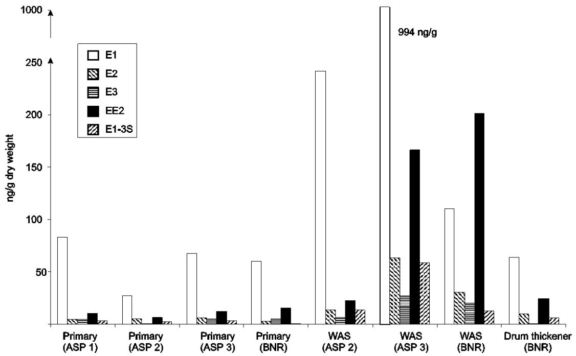
Figure 1. Concentrations of steroid estrogens on primary sludges, WAS and fermented solids from the drum thickener at the BNR works.
