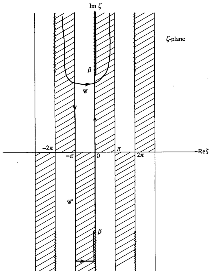
Fig. 1. Diagram of the paths of integration in the \zeta -plane. The shaded regions show where the integral (6) is uniformly convergent. The wavy lines are the branch cuts for the function \mathcal{G}(\zeta) .
