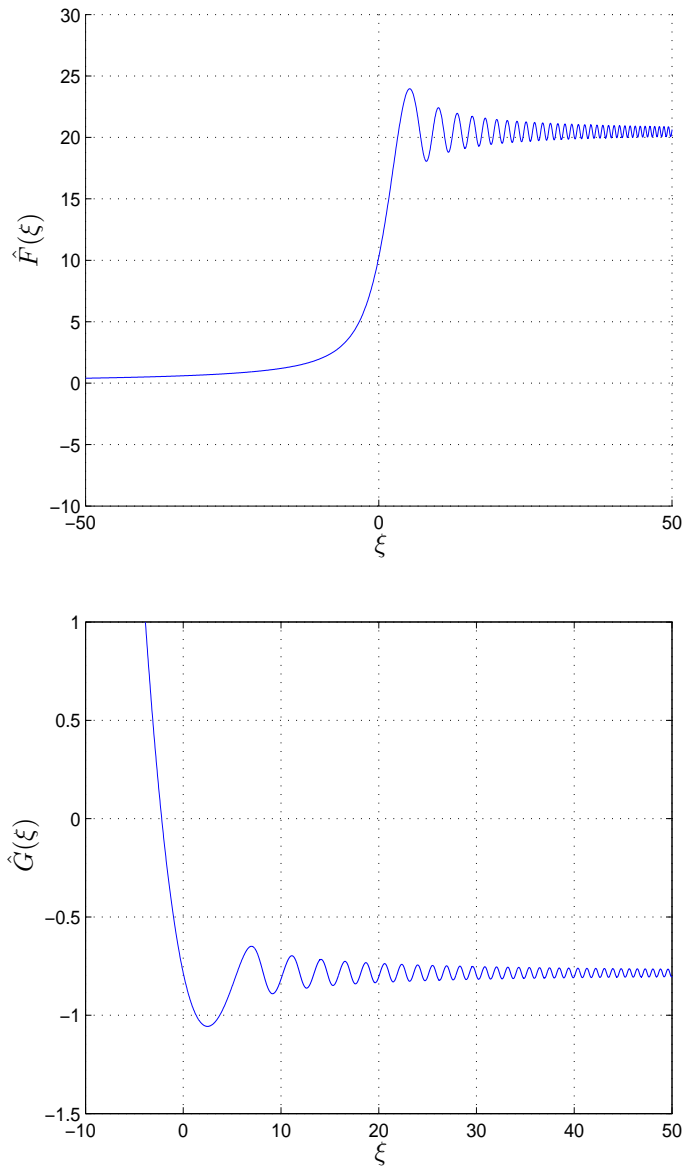
Figure 3: Graphs of \hat{F}(\xi) and \hat{G}(\xi) against \xi . Here F_\infty \approx 20.4 and G_\infty \approx -0.785 .
