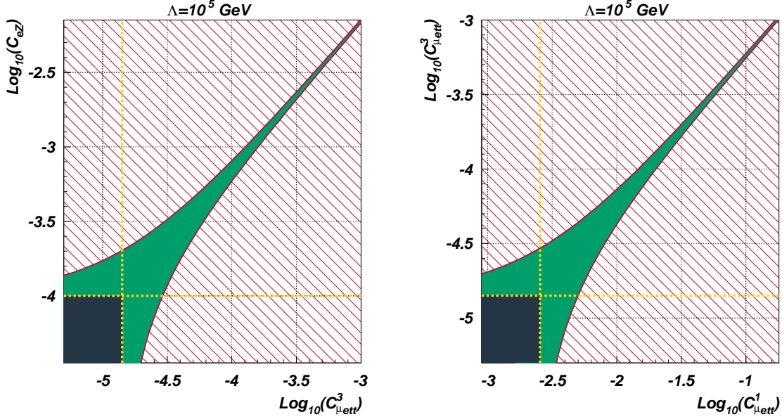
FIG. 2: Correlations between C_{eZ}^{\mu e} and C_{\mu tt}^{(3)} (left) and C_{\mu tt}^{(3)} and C_{\mu tt}^{(1)} (right) at \Lambda = 10^5 GeV. The green area represents the allowed regions if both coefficients are allowed to deviate from zero.
