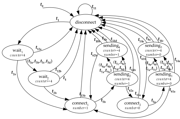
Figure 5. The transformed EEFSM of Initiator process for test generation satisfying all-uses criterion
