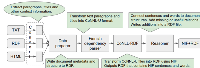
Fig. 1. Pipeline for text processing
