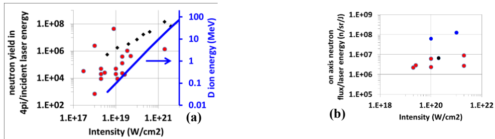
Fig. 23 – (a) In-target Fusion: Experimentally obtained neutron yields [133, 134, 135, 136, 137, 138, 139, 140, 141, 142, 143, 144, 145] (red circles) collected from literature for vs. estimated (black) neutron yield at different laser intensities is shown. Increase in deuterium ion energy from the front surface of a solid deuterated plastic foil, driven by hole-boring mechanism, with increase in laser intensity is shown as blue solid line. (b) Pitcher-catcher setup: Experimentally obtained on-axis neutron flux collected from literature as a function of laser intensity. Red, black and blue dots shows the data obtained for TNSA driven proton and deuterium ions on Li Catcher [145, 146, 147, 148, 149], TNSA driven deuterium ions on deuterium catcher [150] and BOA driven deuterium ions on Cu and Be catcher [151].
