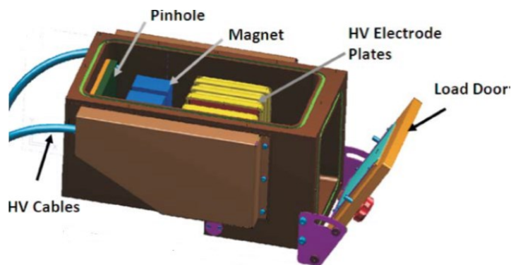
Fig. 27 – Schematic of a Thomson parabola (reproduced with permission from [161]).
