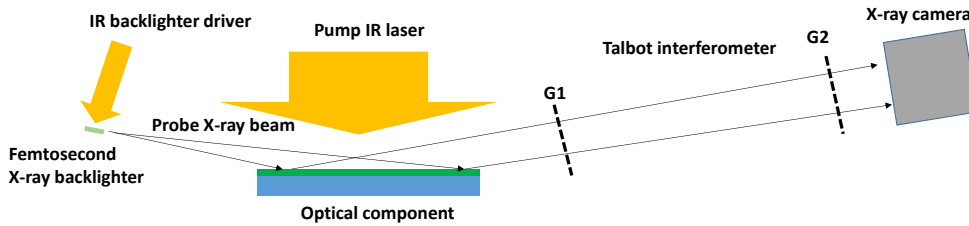
Fig. 5 – Layout of IR pump / X-ray probe diagnostic for time-resolved optical damage studies. G1 and G2 are \mu\text{m} -period transmission and absorption gratings, respectively.
