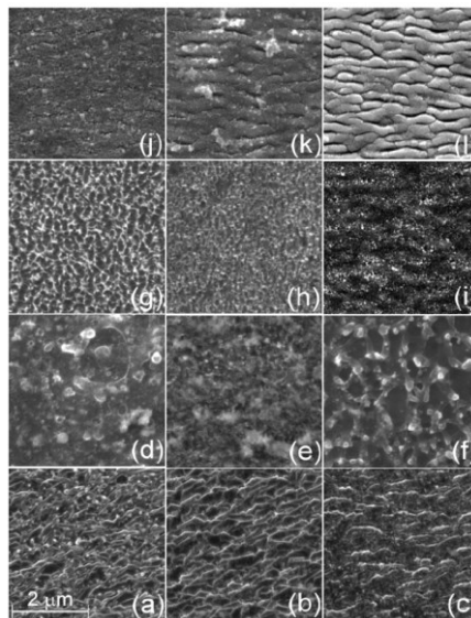
Fig. 8 – Exposed Be samples (images a-f) and W samples (images g-l) in air at atmospheric pressure after 1, 10, 30, 100, 300 and 1000 shots, respectively. (reproduced with permission from [71]).
