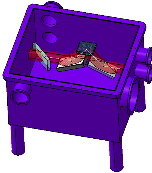
Fig. 13 – CAD model of the implemented adaptive optics and circular polarization system in E5.
