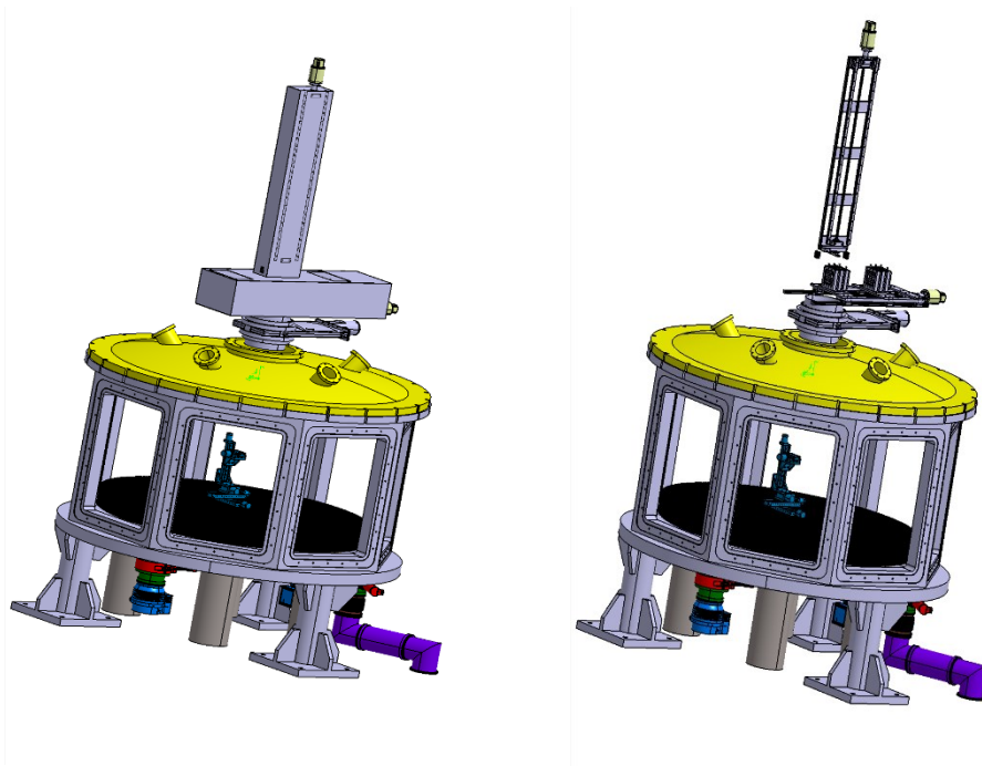
Fig. 12 – 3D CAD design of the load-lock system for solid targets manipulation.
