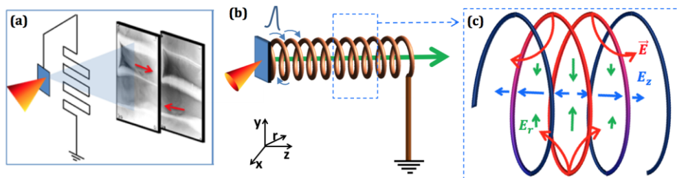
Fig. 19 – (a) shows the setup and data obtained characterizing the charge pulse flowing along a wire connected to the laser irradiated target. (b) Schematic of the target designed for controlling beam parameters of laser driven protons. The helical coil design allows the charge pulse to flow around the proton beam axis, which results in affecting protons of a given range of energies, travelling synchronously with the charge pulse. A schematic snapshot of a small section in the coil is shown in (c) which shows the electric field configuration inside the coil. The red part of the coil represents the segment charged by the travelling pulse at a given moment of time. Where the red arrows represent the electric field lines originating from the coil, the green and blue arrows represent the radial and longitudinal components of the electric field respectively. The length of the green and blue arrows represents relative strength of the field at different locations.
