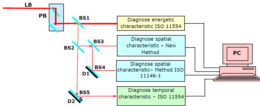
Fig. 3 – Experimental set-up for the laser beam diagnosis. LB – laser beam, PB – positioning beam (generally mirrors for testing the reflectivity, transmission, absorption), BS 1,2,3,4,5 – beam splitters, D 1,2 – dumpers, PC - personal computer.
