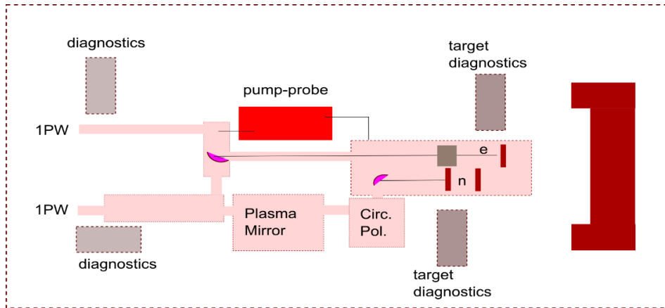
Fig. 10 – Schematic of a proposed interaction chamber in E5 for laser-driven secondary beams.
