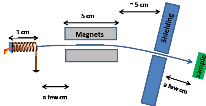
Fig. 21 – A schematic (not to scale) of the experimental setup using magnets to steer the pencil beam of narrow energy bandwidth protons coming out of the coil target. In this case the shielding can be placed obliquely in order to obscure the direct line of sight from the laser interaction. This setup will therefore allow an extremely clean irradiation environment. Tentative dimensions and separation between different objects are mentioned.
