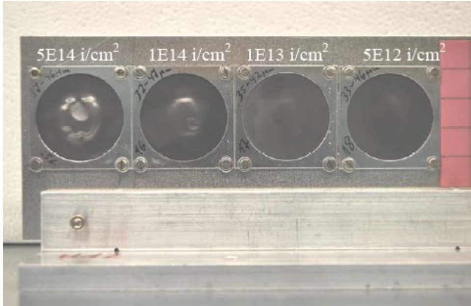
Fig. 1 – Failure of graphite target foils exposed to 5 \times 10^{14} \text{ }^{238}\text{U} ions/cm 2 , 150 \mu\text{s} pulse length, 0.4 Hz, 4.8 MeV/u.
