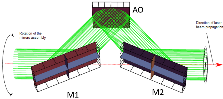
Fig. 14 – Side view of the circular polarization system.
