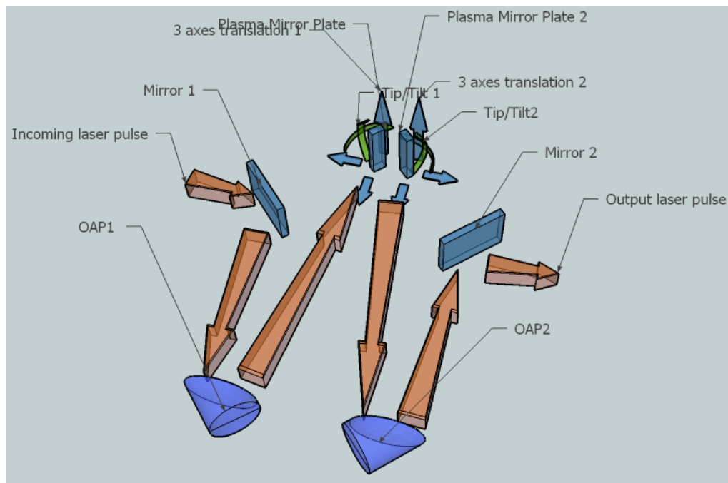
Fig. 16 – Schematic of a double plasma mirror system to be used in the E5 experimental room.
