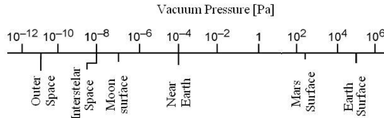
Fig. 2 – Average pressures in the solar system (reproduced with permission from [26]).
