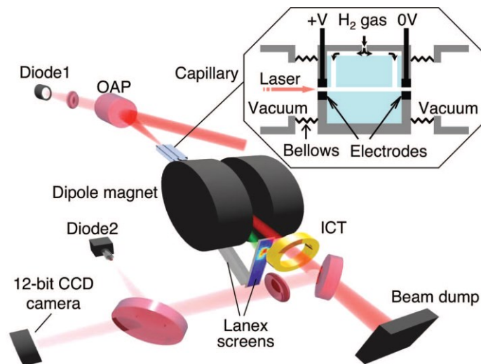
Fig. 25 – Schematic description of a 1.2 T magnetic spectrometer with an energy range 0.03-1.1 GeV (reproduced with permission from [160]).
