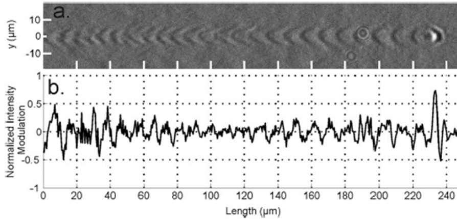
Fig. 29 – Image of a laser-driven plasma wave obtained with a few-cycle probe pulse, (reproduced with permission from [162]).
