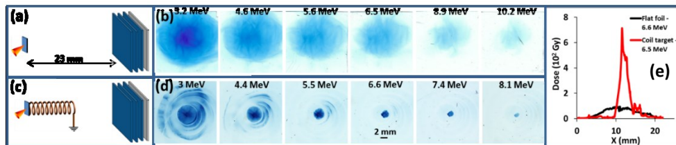
Fig. 20 – (a) and (c) shows the schematic of the experimental setups for the reference flat foil and the proposed coil target respectively. (b) and (d) shows the proton beam profile obtained over different layers of detectors (corresponding to different beam energy) for the case (a) and (c) respectively. (e) shows the comparison between the horizontal lineouts across the proton beams obtained in the 4 th layer of (b) and (d).
