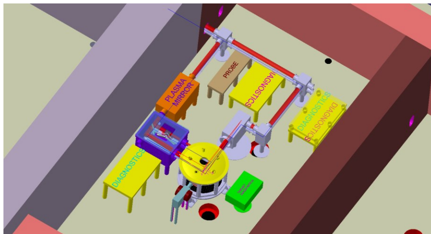
Fig. 11 – CAD design of E5 experimental area.
