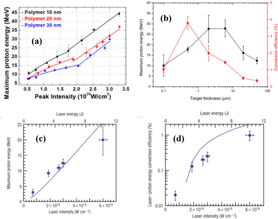
Fig. 18 – Graphs (a) and (b) show the recent experimental data on maximum proton energy produced from the interaction of petawatt class laser with thin foils. (c) and (d) show previously reported scaling for proton energy and conversion efficiency with respect to laser intensity and energy (reproduced with permission from [126, 127]).
