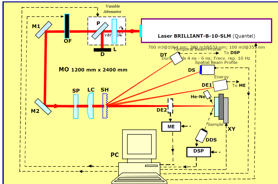
Fig. 4 – L, half wave plate; P, thin film polarizer at incident angle 45^\circ ; D, dumper for laser beam; OF, shatter for high energy laser beam; M1; M2, high reflectivity optical mirrors at 45^\circ incident angle; SP, polarization selector: half wave plate; LC, convergent lens; SH, holographic beam splitter; DT, detector temporal beam profile; DS, detector spatial beam profile FireWare BeamPro model 2523; DE1, energy detector laser beam (measurement range 0,1 mJ – 10 J); DE2, energy detector laser beam (measurement range 0,005mJ – 2 J); ME, two channel energy monitoring; DSP, high speed digitizer (2 Gsa / s) of 10 bit, with high speed signal processor (FPGA structure); XY, motorised translation stage system for displacement and positioning the sample in the laser beam; DDS, detector damage sit: module photodiode C10439-03 with active aperture of 10 mm x 10 mm (HAMAMATSU) and lens with negative aperture; PC, personal computer.
