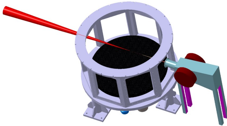
Fig. 26 – 3D CAD design of the interaction chamber and electron spectrometer in the long focal length (F/20) configuration.
