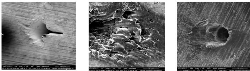
Fig. 6 – SEM image of a W sample after direct irradiation
