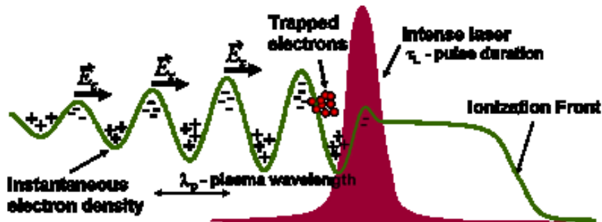
Fig. 17 – Schematic of the interaction of a laser pulse with a neutral, low atomic number gas.
