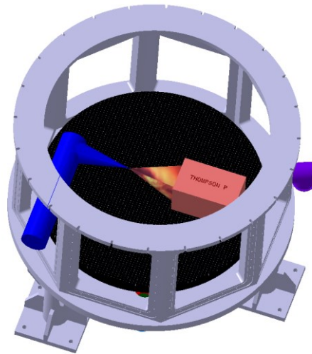
Fig. 28 – 3D CAD design of the interaction chamber in the short focal length configuration and the Thomson parabola for proton/ion diagnostic.
