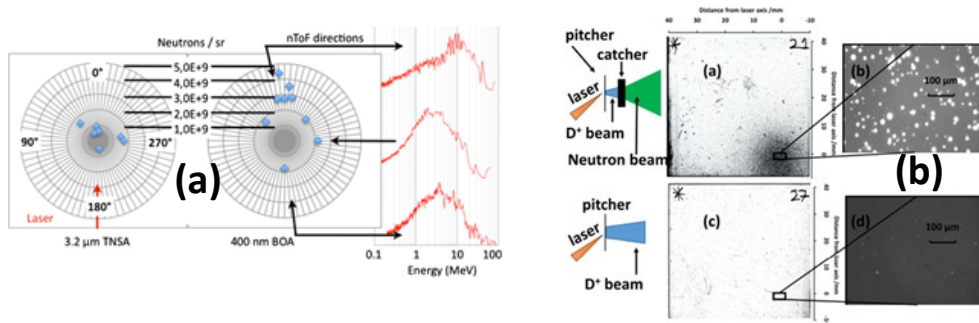
Fig. 24 – (a) and (b) shows recent experimental data showing beamed neutron emission from pitcher catcher configuration employing high energy projectile ions, (reproduced with permission from [151] and [150] respectively).
