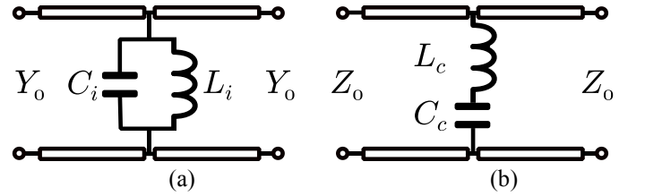
Fig. 1. FSS circuit model: (a)-inductive, (b)-capacitive.
