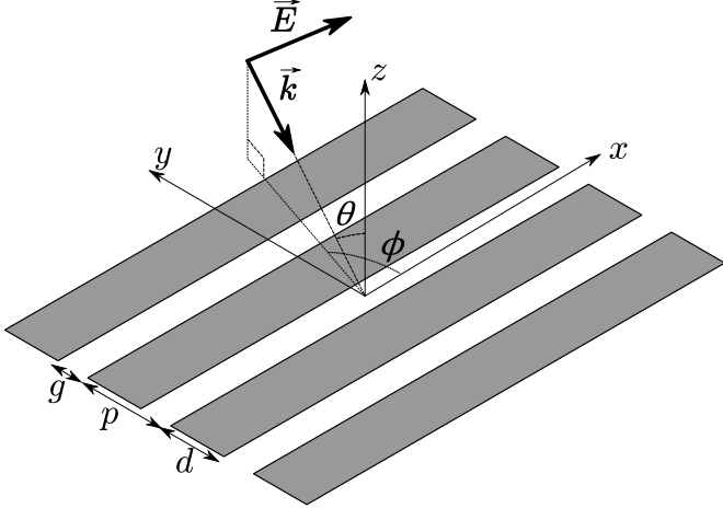
Fig. 2. Strip grating.
