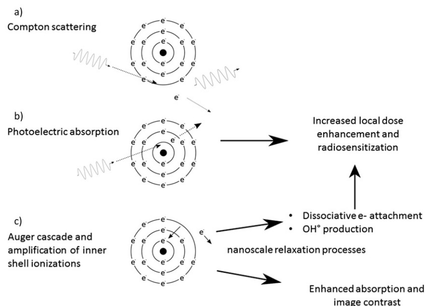
Figure 1. Schematic representation of radiation interactions when an incident photon interacts with a high atomic number ( Z ) material and their downstream applications in radiotherapy. (a) Compton scattering occurs when an incident photon is scattered by a weakly bound outer-shell electron causing the photon to be deflected and lose energy, which is then transferred to the electron that is ejected from the atom. (b) Photoelectric ionization occurs when an incident photon is fully absorbed by an inner-shell electron, transferring its energy to it and causing it to be ejected from the atom. (c) Outer-shell electrons can fall into this vacancy, liberating further energy, often in the form of additional secondary Auger electrons.
