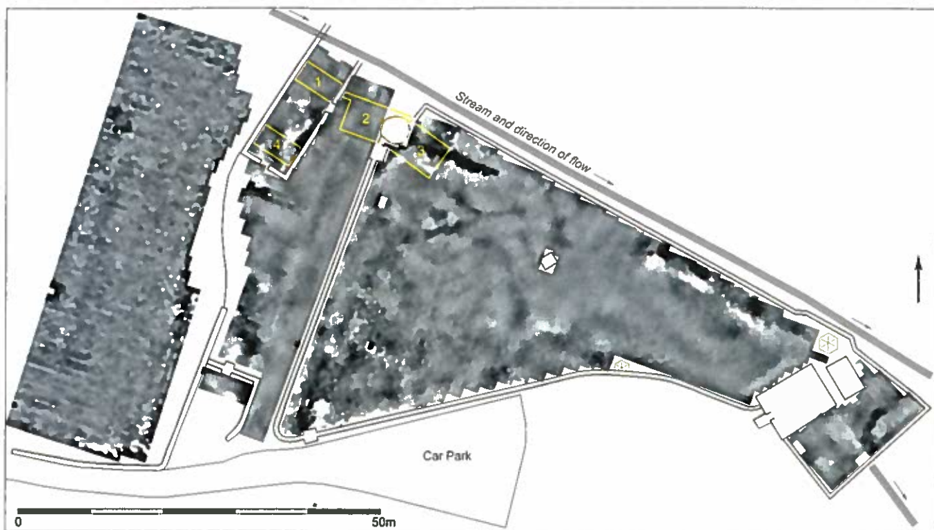
Fig. 7.3—Struell Wells: shade plot of electrical resistance data following application of high-pass filter. Locations of excavation trenches also shown—trenches 2 and 3 on either side of Drinking Well; trenches 1 and 4 within ruins of church.
