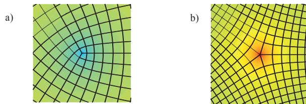
Fig. 1. (a) a negative singularity; (b) a positive singularity. The scalar field shown is a harmonic function representing a continuum description of the quad mesh. It relates to the exponential of isotropic element sizes.
