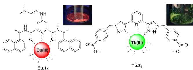
Figure 1: Structures of ligand 1 and 2 and complexes with Eu.1 3 and Tb.2 3 . Inset: the emission arising from solid complexes irradiated under λ = 254 nm.
