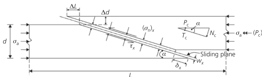
Figure 5. Concrete softening mechanism
