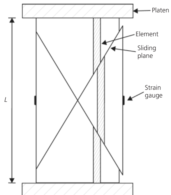
Figure 9. Concrete compression test
