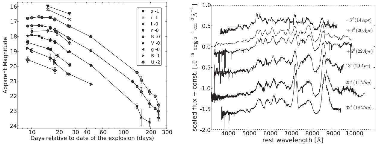
Figure 1. Left: photometry of SN 2012hn in UBgVrIz . The date of the explosion has been fixed 12 \pm 3 d before R -band maximum light ( JD_{\text{exp}} = 245\,6022.5 ). Right: full sequence of photospheric spectra collected for SN 2012hn.
