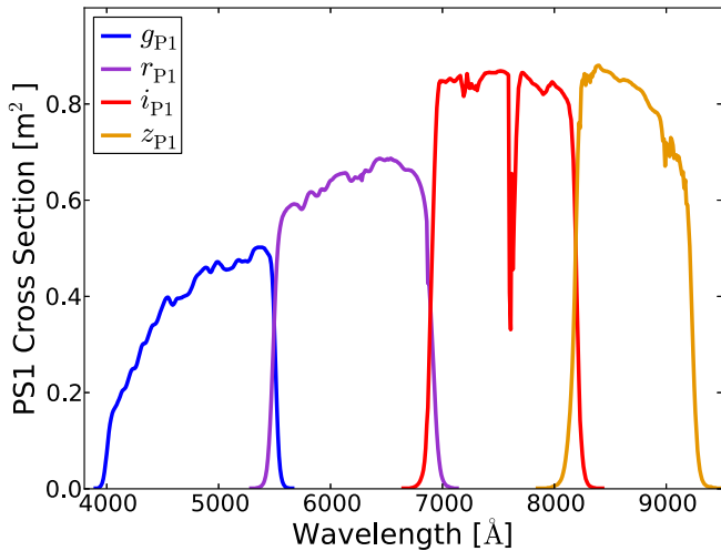
Figure 9. System response function for the four Pan-STARRS1 filters gri_{z_{P1}} at an air mass of 1.2, assuming representative precipitable water vapor and aerosol exponent parameters of 0.65 cm and 0.7, respectively (T12b).
