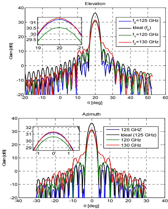
Fig. 7 Simulated radiation patterns (elevation and azimuth planes) of the prototype designed at 125 GHz for the beam scanned and collimated in the direction, \theta=20^\circ , \phi=0^\circ . Frequencies: 120, 125 and 130 GHz.
