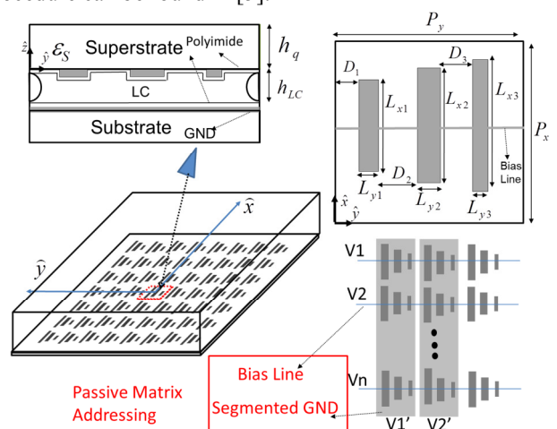
Fig. 1 LC-based Reflectarray. Structure for passive voltage addressing.
