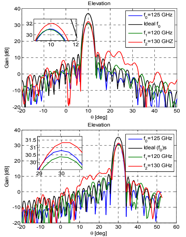
Fig. 8 Simulated radiation patterns (elevation plane) of the prototype designed at 125 GHz for the beam scanned and collimated in the directions, \theta=10^\circ , \phi=0^\circ and \theta=30^\circ , \phi=0^\circ . Frequencies: 120, 125 and 130 GHz.
