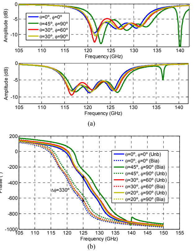
Fig. 6 Simulated (a) amplitude and (b) phase of the reflection coefficient as a function of frequency for different angles of incidence and the two extremes states of permittivity for the prototype 2.
