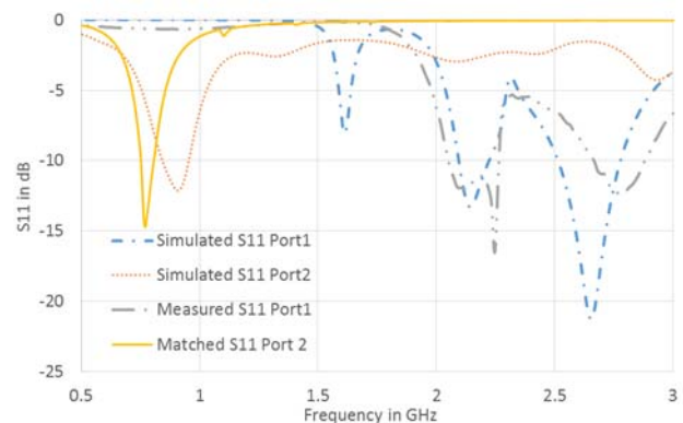
Fig. 2 Return loss
