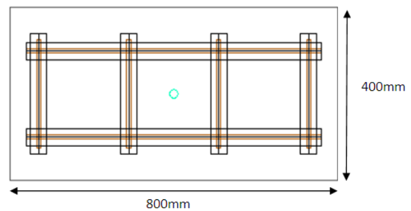
2(a) Plan view of slab 1 showing position of anodes/cathodes Light green circle shows the location at which the sacrificial anode was installed in Phase 3.
