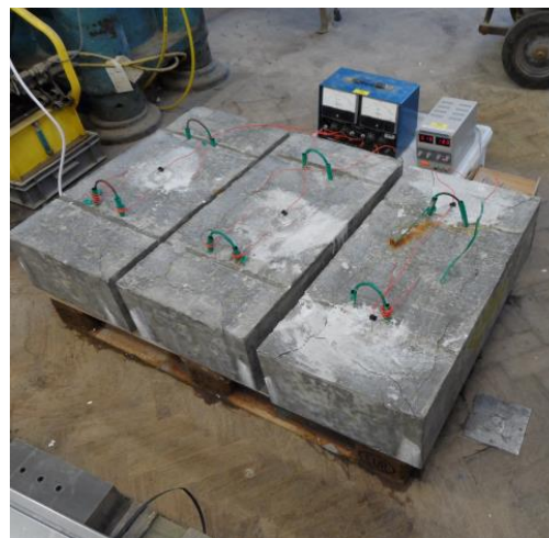
Figure 4. Slabs undergoing accelerated corrosion
