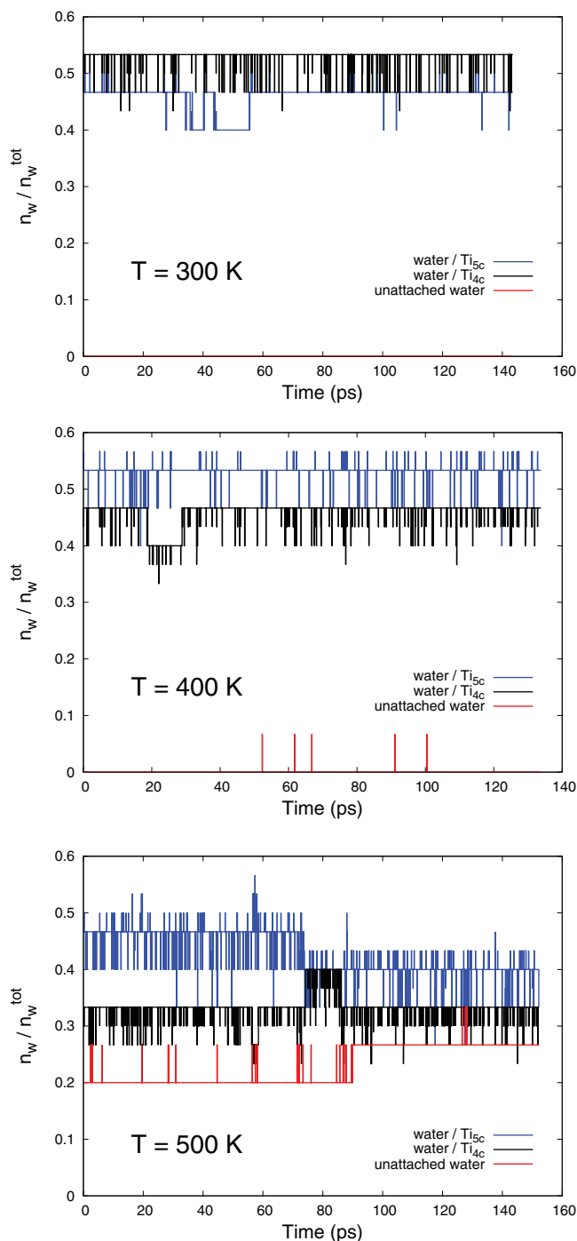
FIG. 6. Fraction of water molecules, n_w/n_w^{\text{tot}} (where n_w^{\text{tot}} = 15 ) adsorbed on 5-fold coordinated titanium atoms Ti 5c (blue line), 4-fold coordinated titanium atoms Ti 4c (black line), and of unattached molecules (red line) collected along the trajectory of three NVT simulations at 300 K (top panel), 400 K (middle panel), and 500 K (bottom panel). See Table VII for the average quantities.
