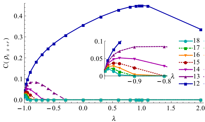
FIG. 2. (Color online) Concurrences of a reduced state of two nonadjacent spins (x, x + r) . For N \gg 1 all the concurrences collapse to the same value: 1/(N - 1) close to the isotropic ferromagnetic point ( \lambda = -1^+ ). The reduced density matrices have been calculated using DMRG simulations with N = 192 . For convenience the spin arrangements are denoted as 12, 13, ... (corresponding to a pair of nearest-neighbor spins, next to nearest-neighbor spins, etc.); however, the entanglement is studied close to the middle of the chain. In the chain of length N the spins correspond to x, x + 1, x + 2, \dots with x = N/2 - 3 . The plotted quantity is dimensionless.
