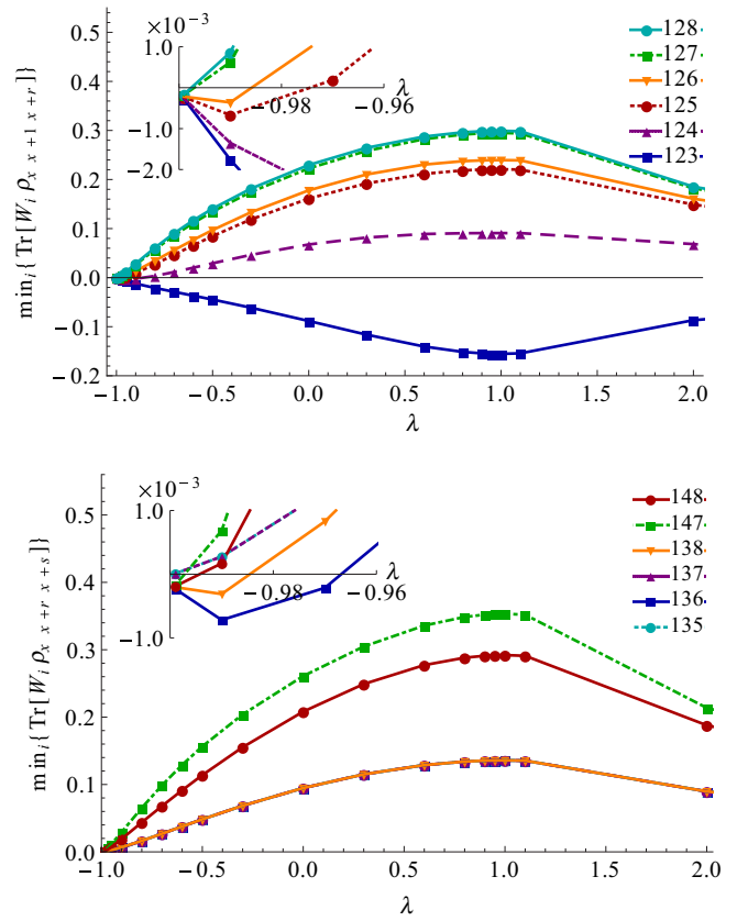
FIG. 3. (Color online) Mean value of the rotationally invariant entanglement witness detecting genuine tripartite entanglement for reduced states of three nonadjacent spins (a) (x, x + 1, x + r) and (b) (x, x + r, x + s) . As \lambda \rightarrow -1^+ (see the insets) GME is detected in all the arrangements depicted in (a), and those shown in (b) except for (135), (137). The reduced density matrices have been calculated using DMRG simulations with N = 192 . For convenience the spin arrangements are denoted as 123, 135, ...; however, the entanglement is studied close to the middle of the chain. The plotted quantities are dimensionless.
