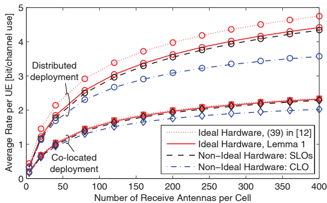
Fig. 4. Achievable rates with MRC filter and either ideal hardware or imperfections given by (\kappa, \xi, \delta) = (0.0156, 1.58\sigma^2, 1.58 \cdot 10^{-4}) . Co-located and distributed antenna deployments are compared, as well as, a CLO and SLOs.
