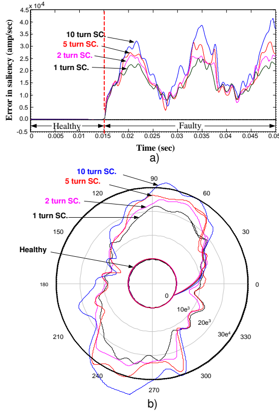
Figure 6. Numerical evaluation; faults considered: 1, 2, 5 & 10 inter-turn short circuits; a) E_{\text{saliency}} respect to time, b) E_{\text{saliency}} respect to the electrical angle (Loci plot).
