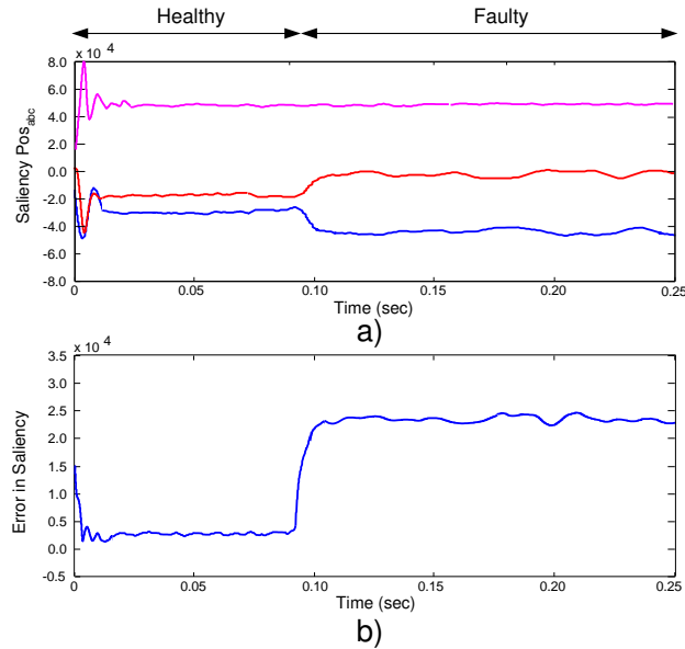
Figure 9: Evaluation under standstill operation, transition between a healthy to faulty system; a) Position estimates ( Pos_{abc} ); b) Error in saliency E_{saliency}
