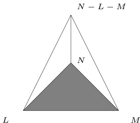
FIGURE 1. The secondary fan for F in 3–2
